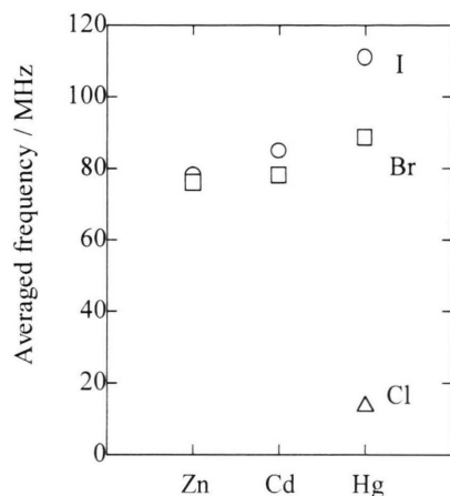
Fig. 3. Comparison of averaged ^{35}\text{Cl} , ^{81}\text{Br} , and ^{127}\text{I} ( m = \pm\frac{1}{2} \leftrightarrow m = \pm\frac{3}{2} ) NQR frequencies in [\text{N}(\text{CH}_3)_4]_2\text{MX}_4 ( M = \text{Zn}, \text{Cd}, \text{Hg}, X = \text{Cl}, \text{Br}, \text{I} ). The NQR frequencies refer to: [\text{N}(\text{CH}_3)_4]_2\text{ZnBr}_4 [13], [\text{N}(\text{CH}_3)_4]_2\text{ZnI}_4 [14], [\text{N}(\text{CH}_3)_4]_2\text{CdBr}_4 [11], [\text{N}(\text{CH}_3)_4]_2\text{CdI}_4 [this work], [\text{N}(\text{CH}_3)_4]_2\text{HgX}_4 ( X = \text{Cl}, \text{Br}, \text{I} ) [12].
