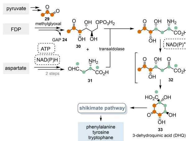
Scheme 6. Alternative biosynthetic pathway to DHQ 33 in the archaea Methanocaldococcus jannaschii .
