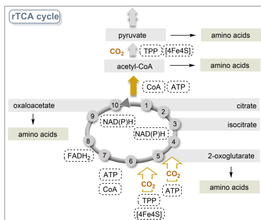
Scheme 2. Overview of reductive TCA cycle with coenzymes and cofactors involved (numbering of intermediates are taken from the TCA cycle in Scheme 1).
