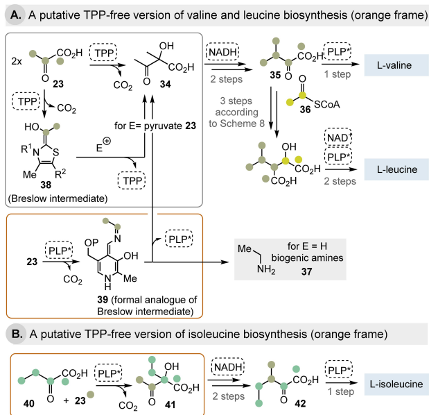
Scheme 7. TPP-mediated biosynthesis of valine and leucine and the hypothetical PLP-mediated analogous conversion (in orange frame) to intermediate 34; B. Analogous hypothetical reaction sequence to isoleucine from 2-oxobutyrate 40 via intermediate 41 (orange frame) and 2-oxocarboxylate 42 (PLP* = pyridoxamine phosphate).
