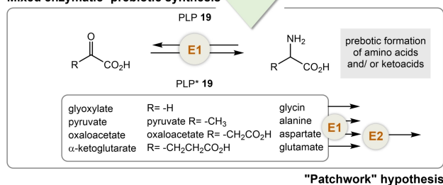
Scheme 10. Merging prebiotic chemistry with concepts of metabolic evolution exemplified for transamination of 2-oxocarboxylic acids (E 1 , E 2 = enzymes).
