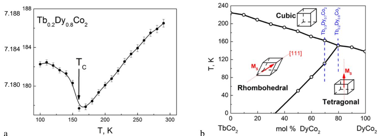
Figure 1. Temperature dependence of Tb_{0.2}Dy_{0.8}Co_2 lattice parameters and phase diagram of TbCo_2 - DyCo_2 [7].
