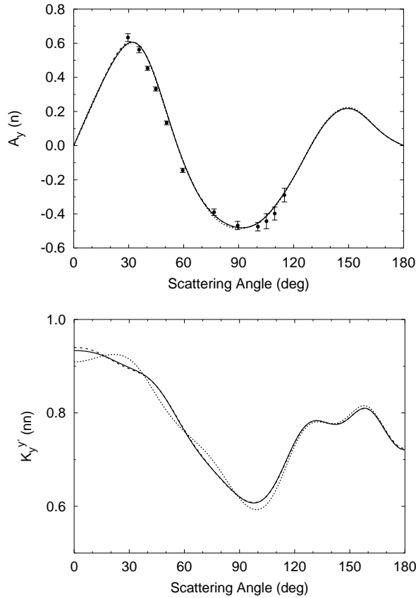
FIG. 8. Nucleon analyzing power A_y(n) and nucleon-to-nucleon spin transfer coefficient K_y^y'(nn) of elastic nucleon-deuteron scattering as function of the c.m. scattering angle at 190 MeV nucleon lab energy. Results including the interaction in partial waves up to two-baryon total angular momentum I=7 (solid curves), I=6 (dashed curves), and I=5 (dotted curves) are shown; differences are only discernible for the observable K_y^y'(nn) . The experimental data are from Ref. [18] and refer to proton-deuteron scattering.
