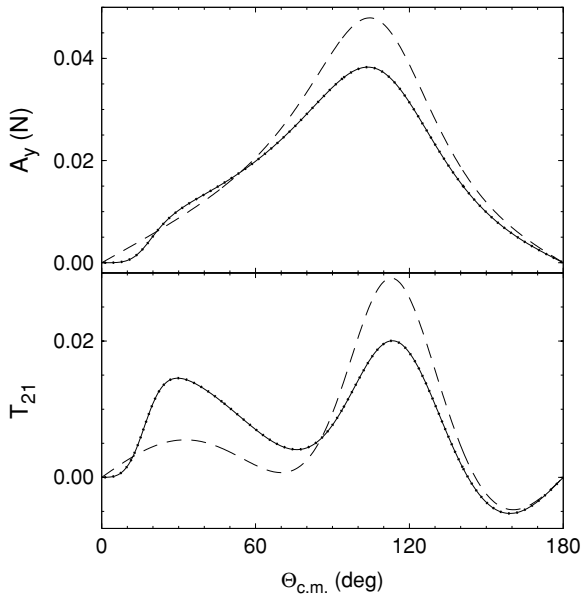
FIG. 1. Nucleon analyzing power A_y(N) and deuteron analyzing power T_{21} for pd elastic scattering at 3 MeV proton lab energy as functions of the c.m. scattering angle. The results of the two new calculational schemes without perturbation theory are graphically indistinguishable and are therefore represented by one curve only, the thin solid one; they are compared with the results obtained using perturbative approach of Refs. [1,2] (thick dotted curves). Results without Coulomb (dashed curves) are given as reference for the size of the Coulomb effect.
