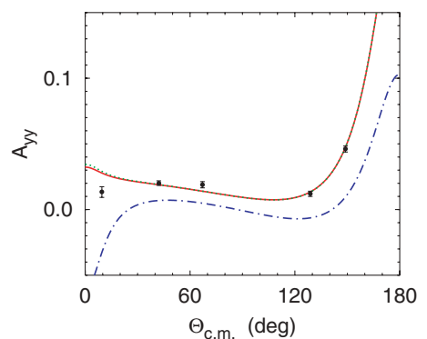
FIG. 3. (Color online) Deuteron tensor analyzing power A_{yy} for pd radiative capture at E_d = 45 MeV as a function of the c.m. d - ^3\text{He} scattering angle. Curves are as in Fig. 1, and the experimental data are from Ref. [27].
