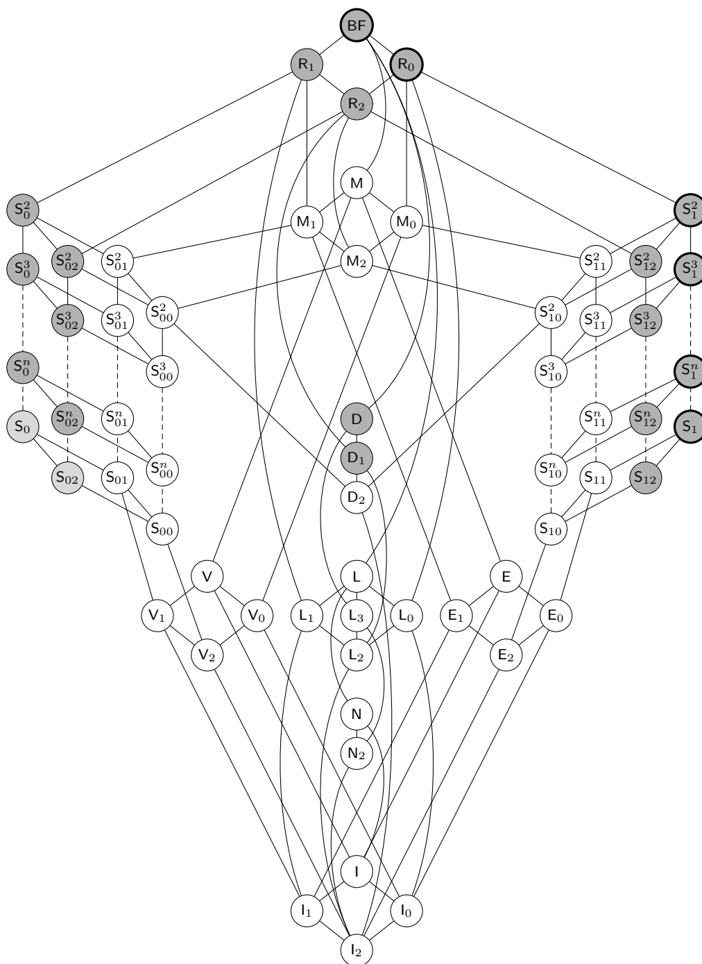
Figure 4.1.1 Post's lattice with our results.
