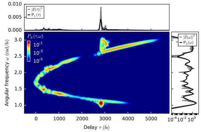
Fig. 4. Analytic signal spectrogram obtained using the balanced optFrog-trace for \sigma^* = 39.1 fs.
