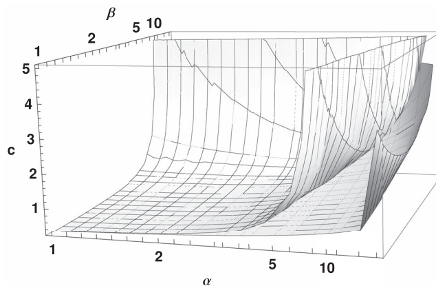
FIG. 3. Comparison of the coherent state uncertainty product (top) and the minimized product using oscillator eigenfunctions up to n = 200 (bottom). Axes scaling as in Fig. 1.
