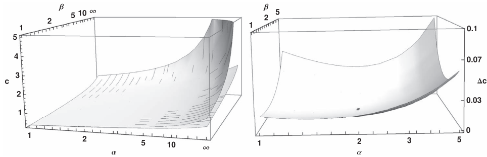
FIG. 2. Left panel: Hirschman's lower bound in comparison with the exact bound. Scaling of axes as in Fig. 1. Right panel: Difference of the two functions around \alpha = \beta = 2 (marked), where the bound is exact.
