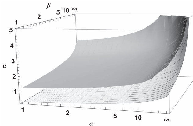
FIG. 1. The constants c_{\alpha\beta} and c'_{\alpha\beta} appearing in Propositions 13 and 12, as determined numerically in Sec. V. The \alpha and \beta axes have been scaled according to \alpha \mapsto (\alpha - 1)/(\alpha + 1) to include the whole range 1 \leq \alpha \leq \infty .
