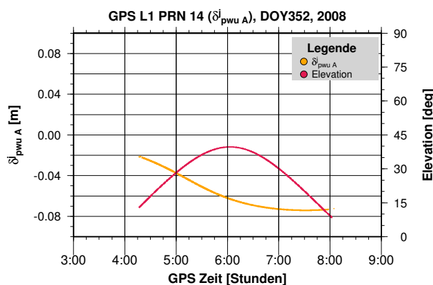
(c) niedrige Elevation
