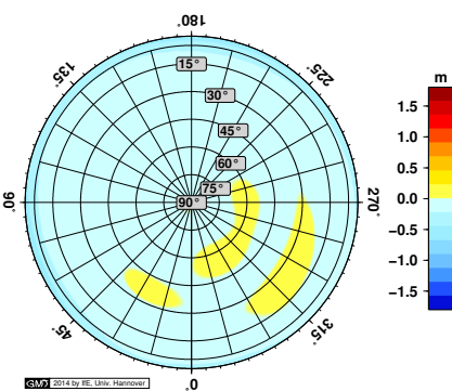
(k) GPS C/A GDV
