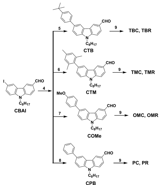
Scheme 4 Synthetic routes for the preparation of phenyl donor based carbazole sensitizers. Reagents: (4) CBAI, (4- tert -butylphenylboronic acid (5) 2,4,6-trimethylphenylboronic acid (6), 4-methoxyphenylboronic acid (7), 4-phenylboronic acid (8), Pd (PPh 3 ) 4 , THF, H 2 O, 70 °C. (9) CBA, CTB, CTM, COMe and CPB, ammonium acetate, acetic acid, 120 °C.
