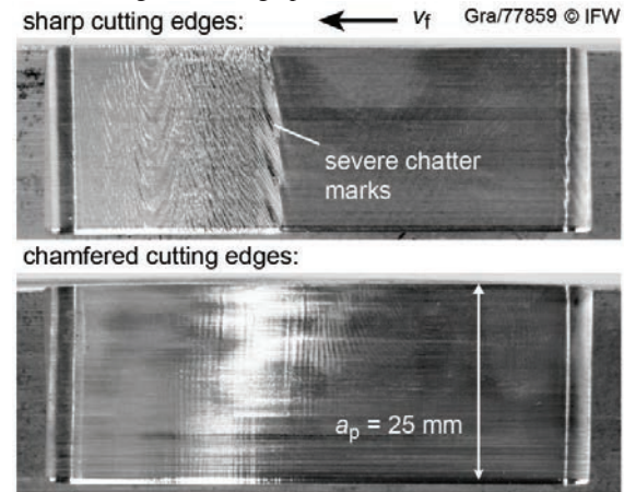
Fig. 5. Comparison of surface finish ( n = 6,000 \text{ min}^{-1} , f_z = 0.08 \text{ mm} )
