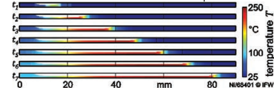
Fig. 7. Simulated temperature distribution in sliced workpiece (chamfered tool, f_z = 0.18 \text{ mm} , n = 4,000 \text{ min}^{-1} )
