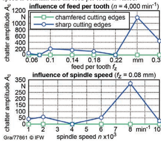
Fig. 4. Intensity of chatter vibrations
