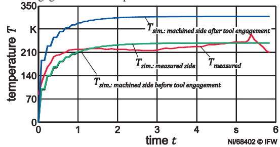
Fig. 8. Maximum temperature (chamfered tool, f_z = 0.18 \text{ mm} , n = 4,000 \text{ min}^{-1} )
