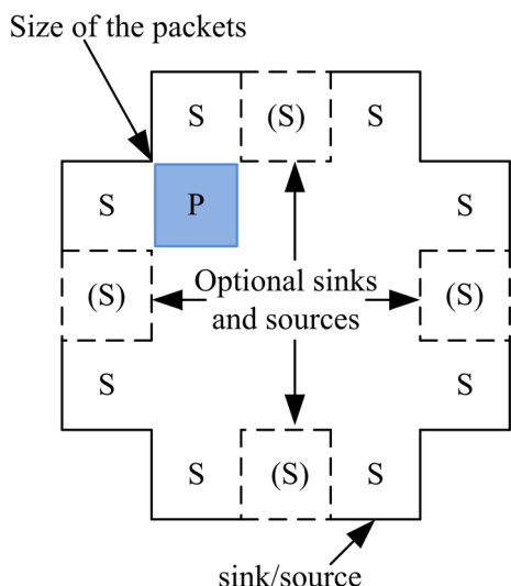
Fig. 13 Conveyor matrix as a hub
