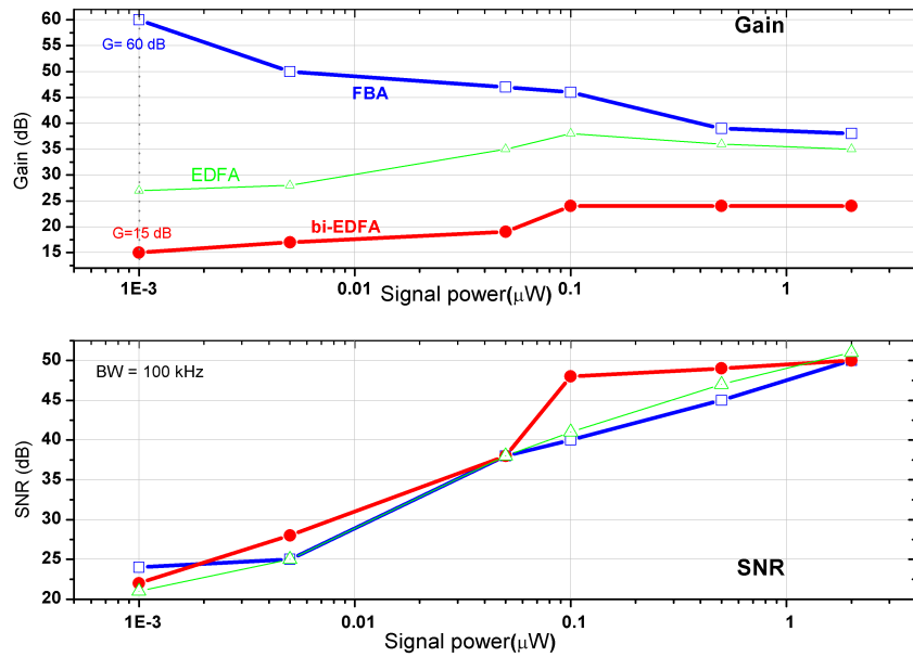
Figure 4.9: FBA in comparison to EDFAs (uni-directional and bi-directional) for different signal powers received at the output of a 25 km fiber: (a) gain (b) SNR. The spectrum analyzer bandwidth is 100 kHz.
