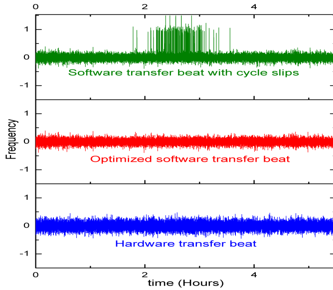
Figure 2.9: The time domain data for the frequency fluctuations of the hardware (blue), an optimized software (red), and cycle slipped (green) transfer beats , NIR-PTB is stabilized to CSL-PTB.
