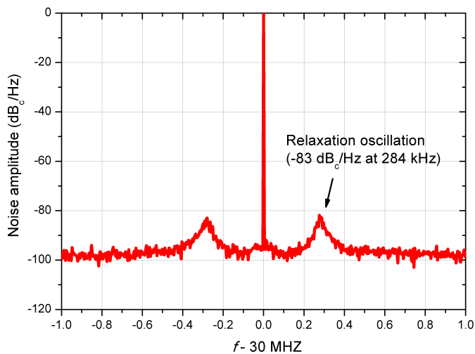
Figure 4.2: Fiber laser Relative intensity noise (RIN), a relaxation oscillation is observed at 284 kHz.
