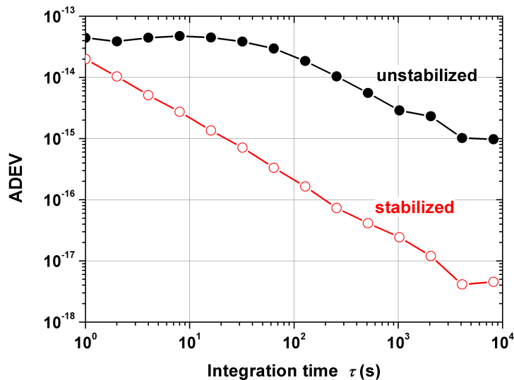
Figure 5.5: Relative frequency instability of the remote beat with the unstabilized NIR laser before (black dots) and after (red open circles) stabilizing the link.
