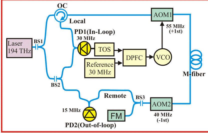
Figure 3.10: Setup for active fiber noise compensation. OC: optical circulator, AOM: acousto-optical modulator, VCO: voltage controlled oscillator, DPFC: digital phase-frequency comparator, TOS: tracking oscillator, PD1: in-loop photodetector, PD2: out-of-loop photodetector, FM: Faraday mirror, and M-fiber: measured fiber.
