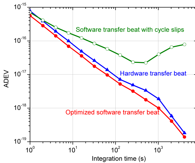
Figure 2.10: ADEV measurement for the hardware (blue triangle), an optimized software (red dots) transfer beats , and a transfer beats with cycle slips (green open circle), NIR-PTB is stabilized to CSL-PTB.
