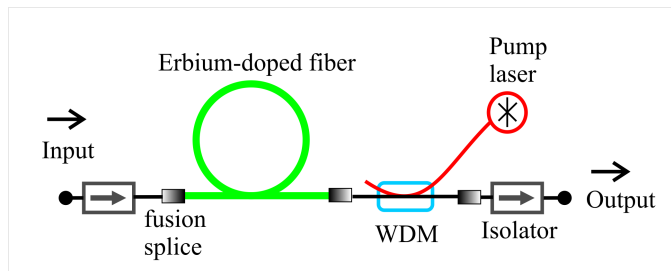
Figure 4.4: EDFA components, WDM: wavelength division multiplexer.
