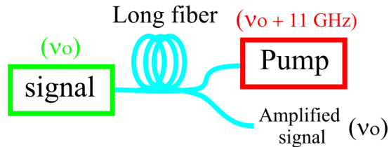
Figure 4.7: FBA amplification setup
