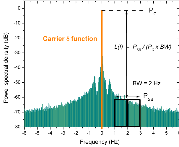
Figure 3.2: The spectrum of a carrier frequency in the presence of noise
