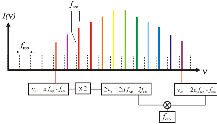
Figure 2.3: Frequency domain representation of frequency comb together with a scheme to detect the carrier offset frequency f_{cco} .
