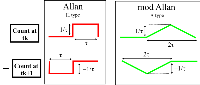
Figure 3.7: (left) AVAR II type, (right) modAVAR \Lambda type weighting functions.
