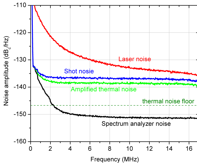
Figure 4.3: Measurement of laser noise, detector thermal noise, shot noise and spectrum analyzer noise.
