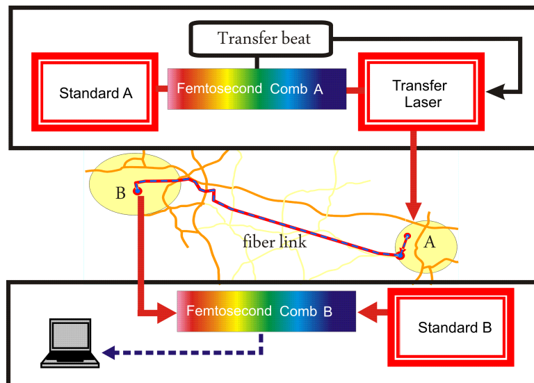
Figure 1.2: Typical remote frequency comparison over optical fiber between a frequency standard at site A and one at site B. A transfer laser at 1.5 \mu\text{m} is used to transfer a stable frequency from one site to the other.
