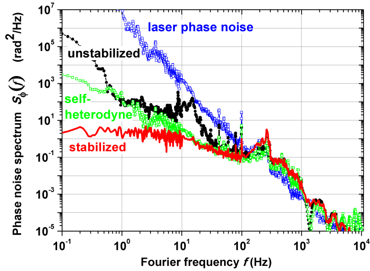
Figure 5.4: Phase noise of the remote beat without stabilizing the NIR laser before (black dots) and after (red line) link stabilization. The phase noise of the free running laser is shown as blue-open squares, and the calculated laser self-heterodyne signal as green open squares.
