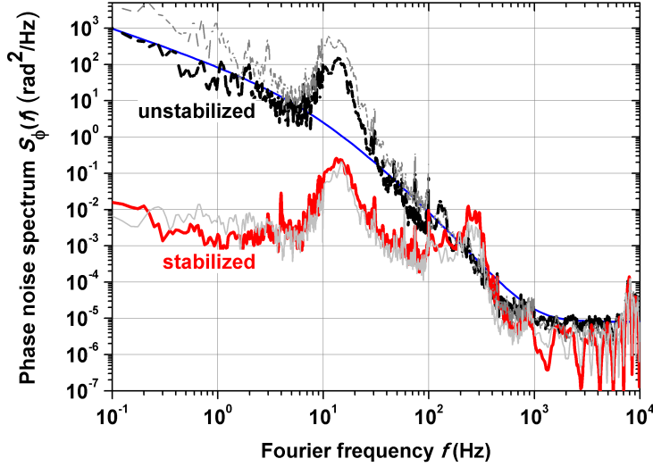
Figure 5.6: Phase noise of the 146 km link: out-of-loop beat before (black-dashed), and after (red-solid) stabilizing the link; in-loop beat: before (gray-dashed), and after (gray-solid) stabilizing the link. Blue line: approximation of S_\phi(f) .
