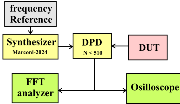
Figure 3.3: Phase noise measurement system; DUT: device under test, DPD: digital phase detector, FFT analyzer: fast Fourier transform analyzer.
