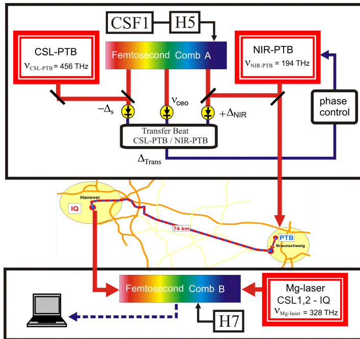
Figure 6.1: Setup for the remote measurement of a Mg-laser at 328 THz against CSL-PTB at 456 THz using a transfer laser (NIR-PTB) at (194 THz) and two frequency combs A and B. The PTB femtosecond frequency comb A is locked to a H-maser (H5) referenced to the Cesium fountain CSF1. At the remote end the transfer beat is calculated from the measured individual beat signals. The IQ femtosecond frequency comb B is locked to an H-maser (H7).
