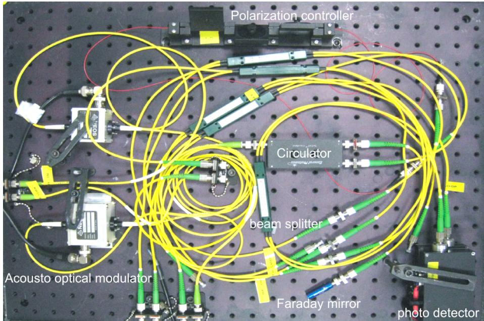
Figure 3.11: All-in-fiber interferometer used to detect and compensate phase noise
