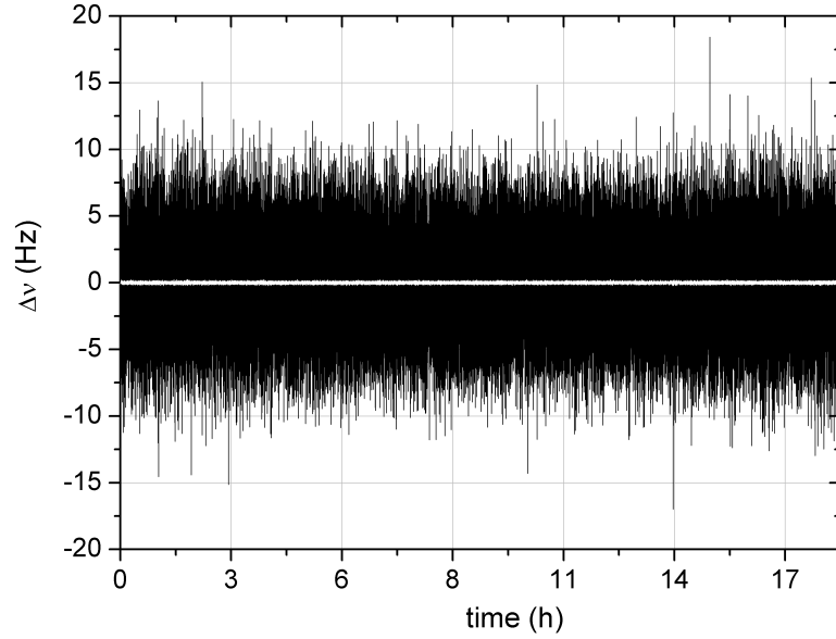
Figure 7.5: Time record of the frequency deviation of the transmitted signal from its nominal value of 15 MHz over a measurement time of 17 hours
