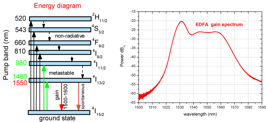
Figure 4.5: (left) \text{Er}^{3+} Energy levels in fused silica fiber, (right) EDFA spectrum.
