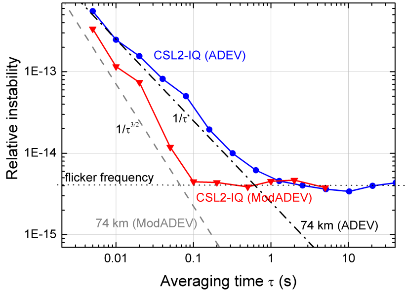
Figure 6.4: Relative instability of the CSL2-IQ laser measured with a \Pi -type frequency counter (blue dots) and with a \Lambda -type frequency counter (red triangle). The instability of the fiber transfer is shown as a black dashed-dotted line for the ADEV and as gray dashed line for the ModADEV.
