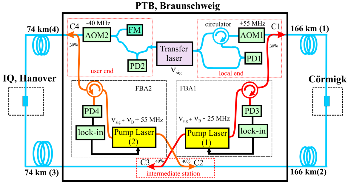
Figure 7.2: : Brillouin amplification in a frequency transfer system, AOM: Acousto-optic modulator, PD: photodetector, FM: Faraday mirror, C1: 30/70, C2: 40/60, C3:40/60, C4:30/70 simple fiber couplers.
