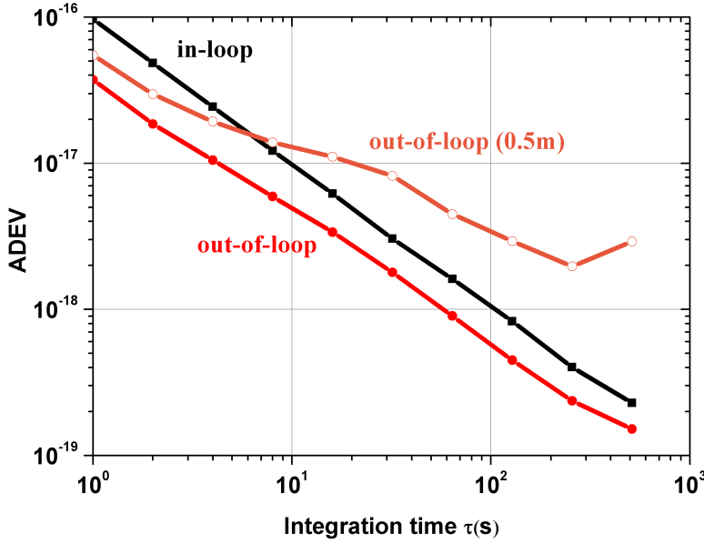
Figure 3.17: Relative frequency instability of stabilized in-loop (black squares) and out-of-loop beats for a symmetrical (red dots) and an unsymmetrical (orange circles) interferometer.
