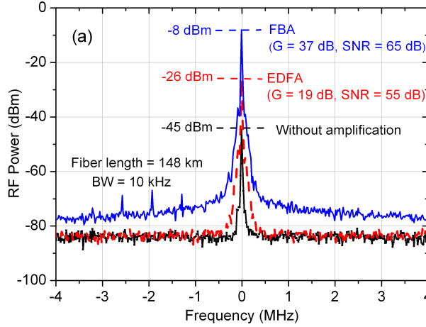
Figure 4.10: Detected heterodyne beat power (RF) obtained with FBA and with bi-directional EDFA, when 5 mW signal power are injected into 148 km fiber ( P_{pump} = 20 mW, \nu_B = 10.974 GHz).
