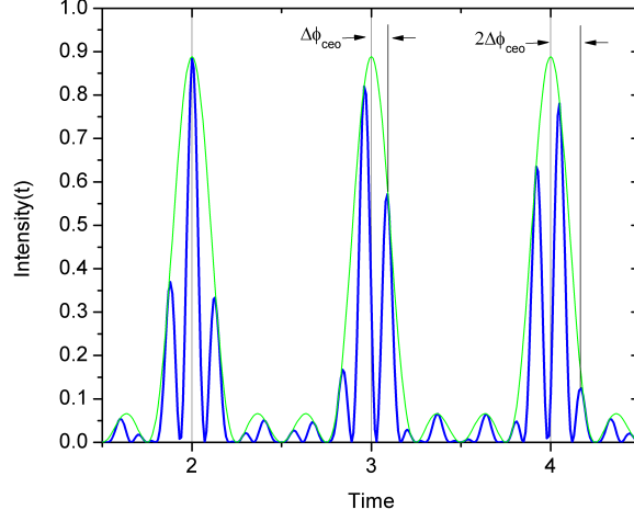
Figure 2.2: Time domain representation of frequency comb. \Delta\phi_{cco} is the offset phase between two consecutive pulses.
