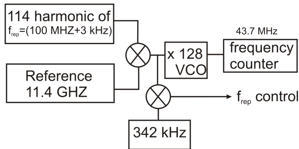
Figure 2.5: Harmonic detection of the repetition rate ( f_{rep} ).
