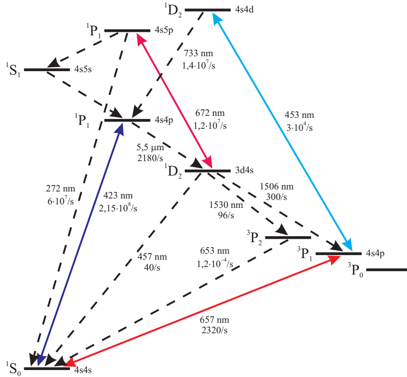
Figure 2.1: Excerpt from the energy level diagram of ^{40}\text{Ca} . The optical transitions which are involved in the cooling scheme are shown as colored lines. The dashed lines indicate spontaneous decays. For the most relevant transitions the wavelengths and the corresponding Einstein A-coefficients are shown.
