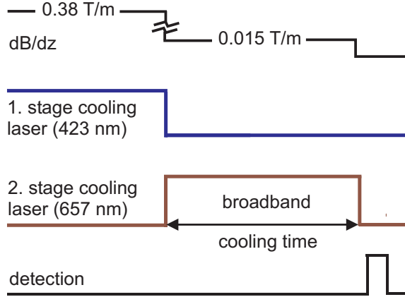
Figure 2.4: Cooling sequence for the preparation of a 12 \mu\text{K} cold sample (refer to the text).
