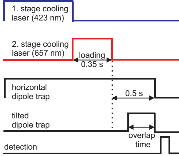
Figure 5.13: Measurement sequence for the investigation of the loading behavior of the dimple.
