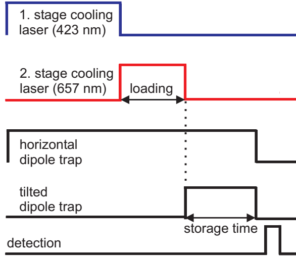
Figure 5.5: Measurement sequence for the crossed-beam optical dipole trap. In comparison to the sequence in figure 5.4 the tilted trap will be overlapped to the horizontal one after switching-off the MOT.
