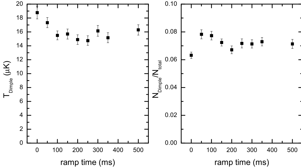
Figure 5.9: Adiabatic generation of the dimple potential. Left: evolution of the ensemble temperature in the dimple as a function of different ramping times and right: the corresponding ratio N_{\text{Dimple}}/N_{\text{total}} (see text).
