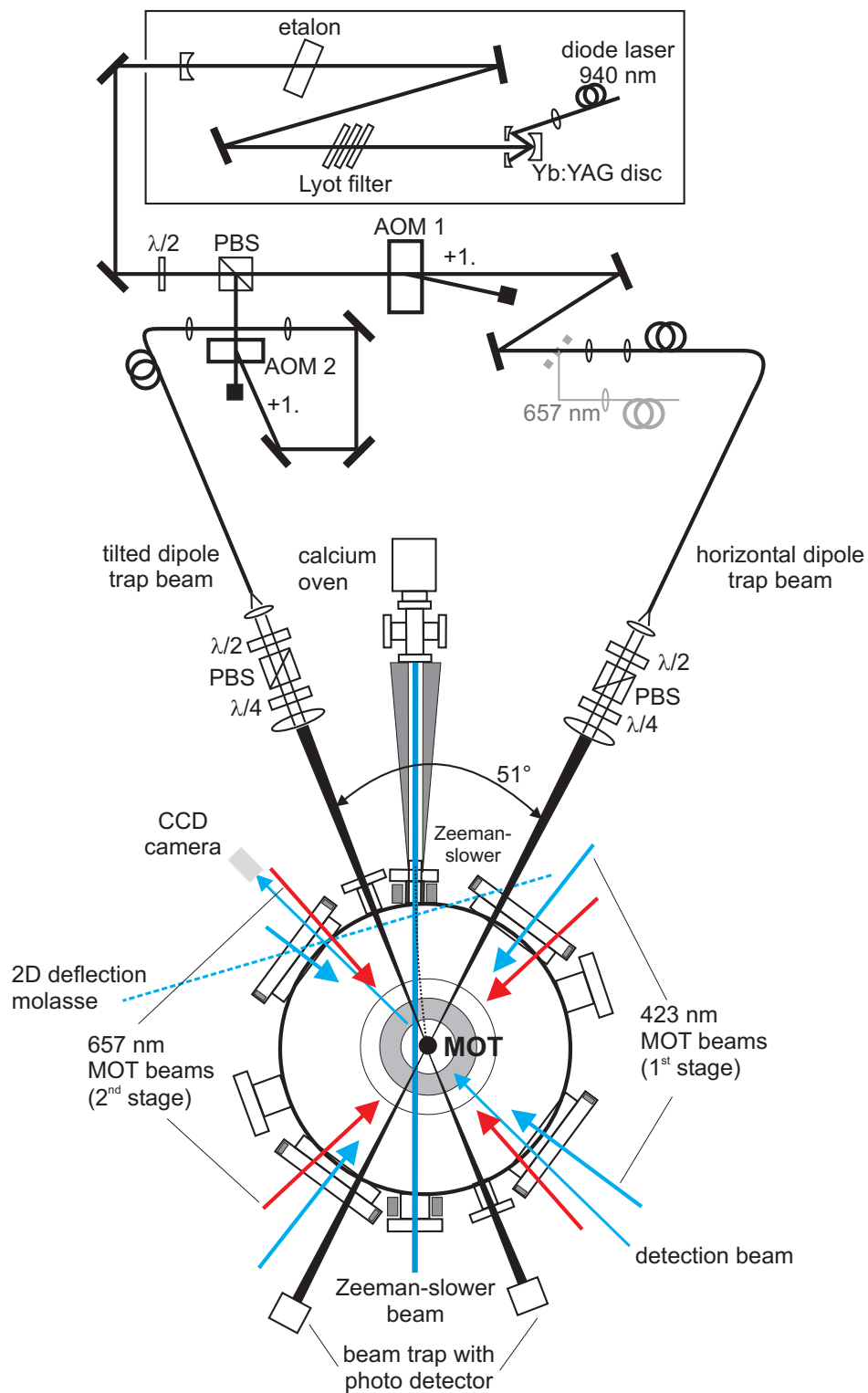
Figure 4.4: Top view of the experimental setup with the beams of the horizontal and tilted dipole trap. This beam is tilted by 20^\circ with respect to the horizontal plane, which corresponds with the drawing plane. An explanation of the different parts is given in the text as well as in Figure 2.2. AOM: acousto-optical modulator, PBS: polarizing beam splitter, \lambda/2 , \lambda/4 : retardation plates.
