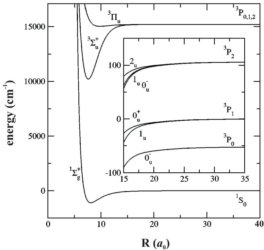
Figure 4.8: Potentials of two calcium atoms as function of the interatomic distance R . At short range the potentials are labeled by their Hund's case (a) symmetry. Inset: close to the 3P+1S asymptote the potentials are described by Hund's case (c) symmetry. Figure taken from Ciuryło et al. [Ciu04].
