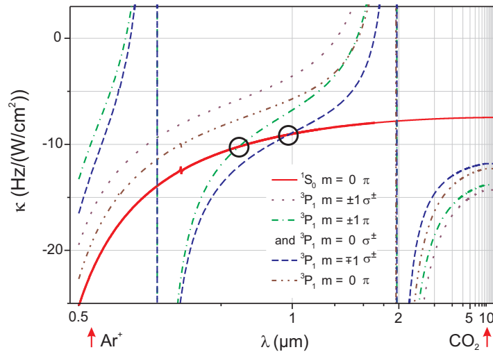
Figure 4.2: Normalized light shifts \kappa for the ground state ^1S_0 and for the excited state ^3P_1 with its Zeeman sublevels m and different polarizations \pi or \sigma^\pm of the dipole trapping laser as a function of its wavelength. At two wavelengths one can observe an equal shift of the ^1S_0 state and of one component of the ^3P_1 state. These are the magic wavelengths indicated by a circle. The vertical lines are due to poles in the polarizability from the transition 4s4p\ ^3P_1 - 4s4d\ ^3D_{1,2} at 1.9\ \mu\text{m} and 4s4p\ ^3P_1 - 4s5s\ ^3S_1 at 612\ \text{nm} .
