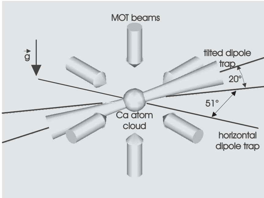
Figure 5.1: Configuration of the two optical dipole traps and the MOT.
