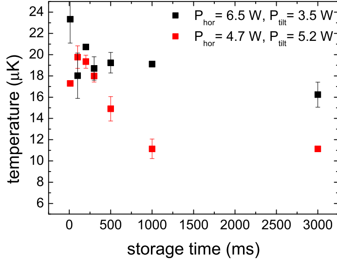
Figure 5.8: Ensemble temperatures in the dimple as a function of the storage time. The black squares indicate the temperatures, which are observed for the atoms stored in a crossed-beam trap with a power of 6.5 W in the horizontal and 3.5 W in the tilted beam. The resulting temperatures for similar powers in the horizontal (4.7 W) and the tilted trap (5.2 W) are indicated by red squares.
