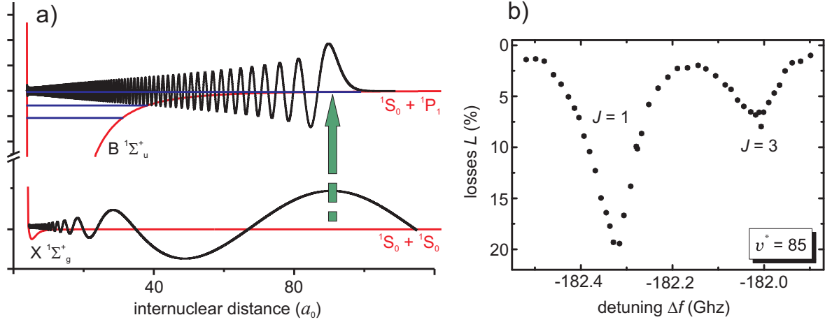
Figure 3.1: Illustration of the photoassociation process. a) A pair of colliding ground state atoms, described by the s -wave scattering function (black curve in the lower part of the figure), is resonantly excited (green arrow) to a bound molecular state (black curve in the upper part of the figure) near the dissociation limit 4s^2\ ^1S_0 + 4s4p\ ^1P_1 . The corresponding molecular potentials of the ground X\ ^1\Sigma_g^+ and excited state B\ ^1\Sigma_u^+ are shown as red curves. The excitation to different molecular levels (blue lines in the upper part of the figure) probes the scattering wave function at different internuclear distances. The internuclear distance is given in units of the Bohr radius a_0 . An example of such a photoassociation spectrum of the vibrational level v^* = 85 below the asymptote of state B\ ^1\Sigma_u^+ is shown in figure b) . The detuning \Delta f is measured with respect to the dissociation limit 4s^2\ ^1S_0 + 4s4p\ ^1P_1 . At a temperature of 1.5 mK transitions to the rotational levels with quantum number J = 1 and J = 3 are observed.
