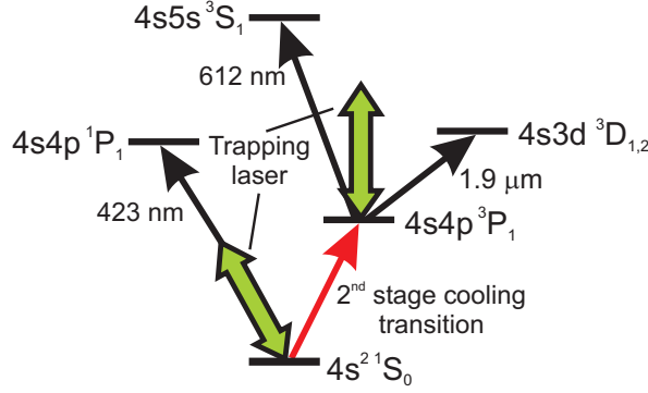
Figure 4.1: The most important couplings of the ^1S_0 and ^3P_1 state, which contribute to their ac-Stark shifts.
