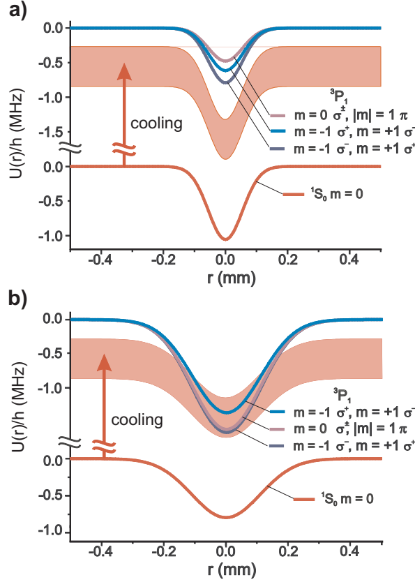
Figure 4.3: The dipole potential of the ground and the excited states as a function of the distance r from the center of the trapping laser beam. In case a) at a wavelength of 514 nm ( \text{Ar}^+ laser) the ^1S_0 state has a bigger shift in comparison to the different states of ^3P_1 . In case b) the opposite situation is considered, realized by a dipole trap at a wavelength of 10.6 \mu\text{m} ( \text{CO}_2 laser). The experimental parameters of case a) are an optical power of 8 W and a beam waist of 110 \mu\text{m} . In case b) a power of 80 W is focused to a beam waist of 220 \mu\text{m} . The band indicates the broadened spectrum of the cooling laser.
