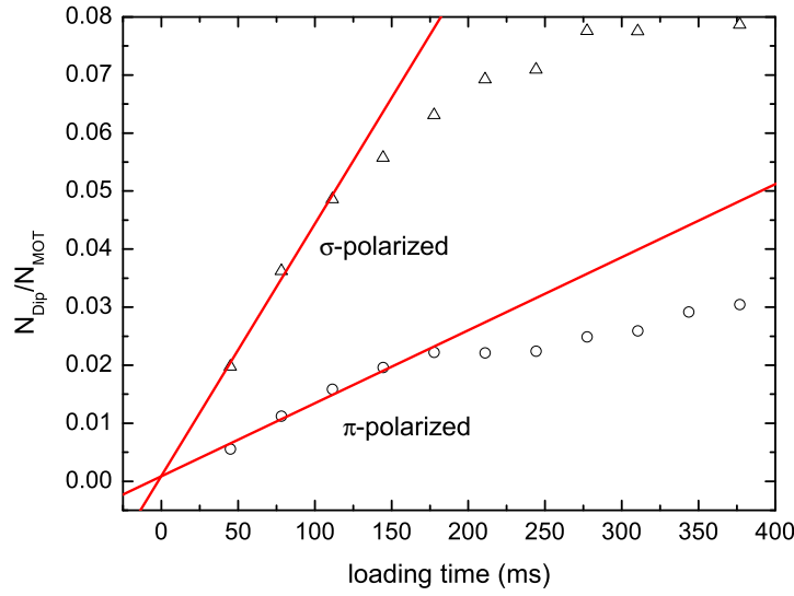
Figure 4.6: Initial loading behavior in a dipole trap realized with linear ( \pi ) and circular ( \sigma ) polarized light. The number of atoms increases linearly in time until loss processes prevail over the loading rate and limit the maximum number.
