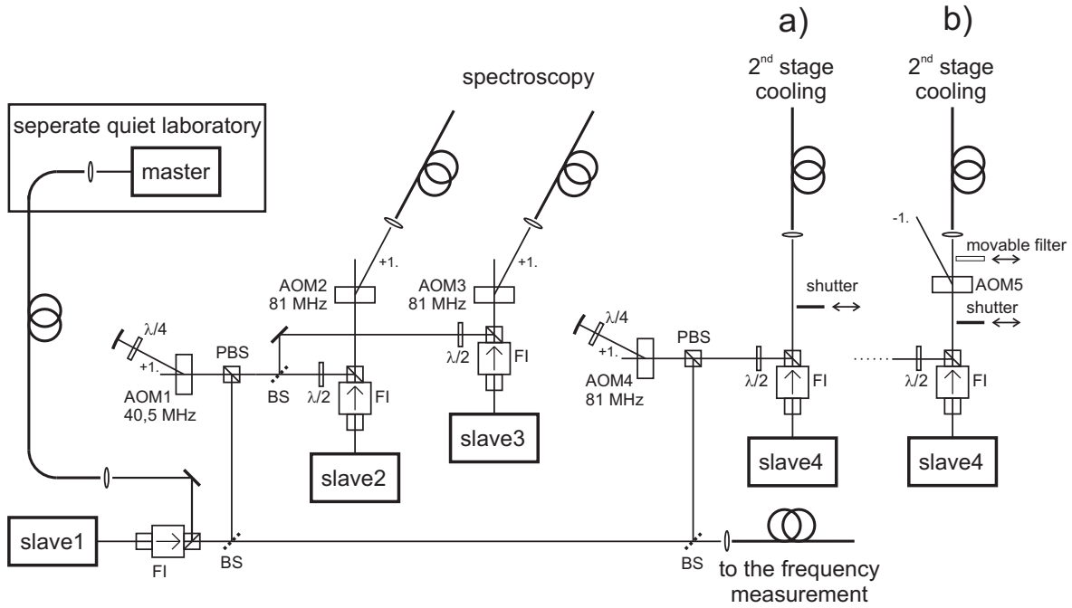
Figure 2.3: The laser system at 657 nm for spectroscopy and the second stage of the MOT. The different slaves are injection locked to the stabilized light of the master. AOM: acousto-optic modulator, FI: Faraday isolator, BS: beam splitter, PBS: polarizing beam splitter, \lambda/2 , \lambda/4 : retardation plates. Second stage cooling without a) and with b) the possibility to reduce the optical power of the cooling light in the zeroth order of an AOM and additionally by a movable filter glass.
