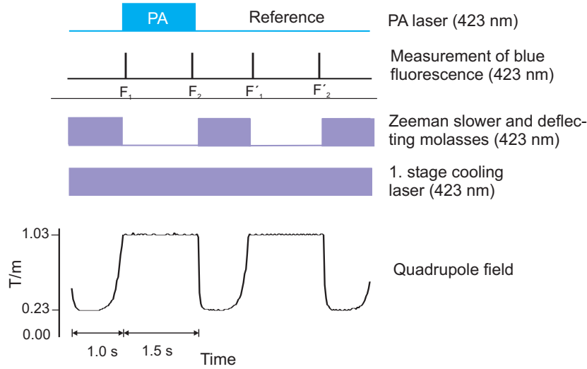
Figure 3.2: Time sequence of the photoassociation measurement. At each detuning with respect to the atomic resonance the measurement consists of two cycles. The MOT is loaded at a low magnetic field gradient and subsequently compressed by increasing the gradient. The loading ends at the high gradient by switching off the Zeeman slower and the molasses. The generation of \text{Ca}_2 starts by shining in the photoassociation (PA) laser for 1.5 s. The blue fluorescence at the beginning and at the end of the PA process is detected ( F_1 , F_2 ) and compared with the respective fluorescence signals without the PA laser ( F'_1 , F'_2 ) in order to calculate the relative PA-induced losses L .
