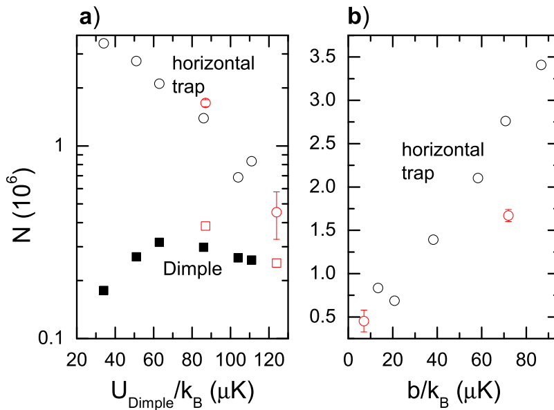
Figure 5.6: Number of atoms in the crossing region and in the horizontal trap plotted against the potential depth of the dimple U_{\text{Dimple}} (figure a)). The number of atoms in the horizontal trap depends on the potential barrier b (figure b)), induced by the overlapping potential of the tilted trap. For trap depths of the dimple around 80 \mu\text{K} the number of atoms reaches a maximum. This is attributed to a limitation in density and a decrease in the reloading from the horizontal trap. The red colored points are from identical measurements realized, if the dimple is loaded without MOT.
