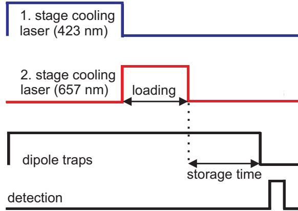
Figure 5.4: Time sequence for the measurements in the crossed-beam dipole trap. After the usual preparation of atoms in the two-stage MOT both dipole traps are loaded. After the storage time an absorption image is taken.
