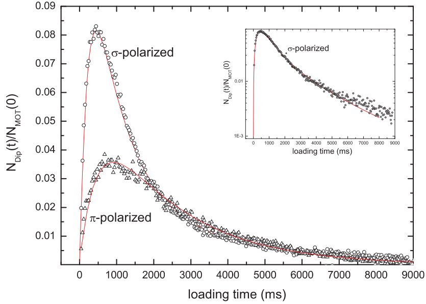
Figure 4.10: Transfer efficiency from the MOT into the dipole trap as a function of the loading time for a dipole trap realized with linear ( \pi ) and circular ( \sigma ) polarized light. The solution of equation 4.9 is fitted to the data (red solid line). For \sigma -polarized trapping light the cooling conditions inside the dipole trap are more like in free space which results in a four times higher loading rate. The maximum of transferred atoms is limited by light assisted collisions (see text). For loading times longer than 6 s the number of remaining atoms is slightly higher than described by the model (see inset).
