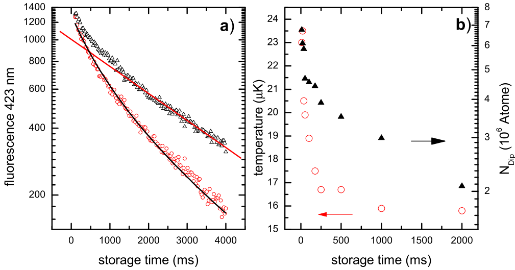
Figure 4.7: a): Decay of atoms from the dipole trap as a function of storage time, without any MOT light (black triangles) and with the MOT light on (red circles). No influence on the decay is observed, if the quench light is irradiated in addition to the MOT light. The black solid line is a fit according to equation 4.8. The red solid curve describes the exponential decay ( 1/\gamma_{\text{Dip}} = (3.6 \pm 0.1) s) after the hottest atoms are escaped from the trap, which is shown in b): The temperature (red circles) decreases during \approx 1 s until a value around 16 \mu\text{K} is reached. The corresponding number of particles are denoted by the black triangles.
