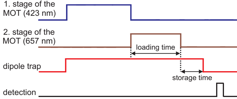
Figure 4.5: Time sequence for the measurements with the dipole trap. The focus of the dipole trap laser beam is superimposed on the MOT in space and time. After the usual preparation in the 423 nm MOT the loading into the dipole trap becomes significant as soon as the temperature of the ensemble in the 657 nm MOT is low enough. When the loading of the trap is finished and the 657 nm MOT is switched off, the atoms are stored for variable times. The detection of the atoms is performed by taking absorption images or by measuring the fluorescence light.
