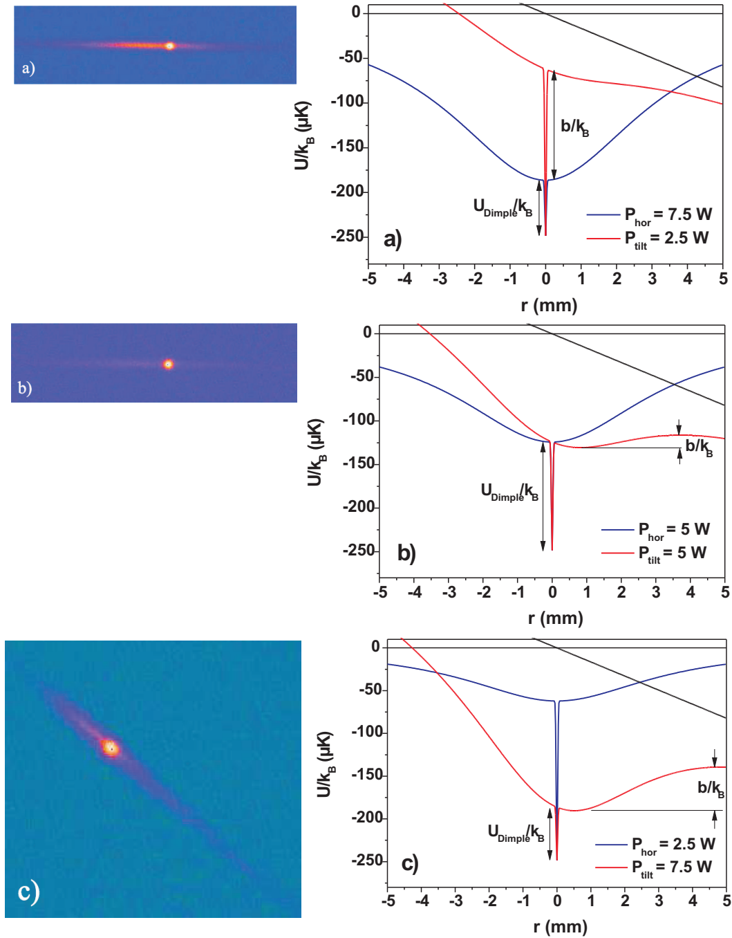
Figure 5.3: The potential of the crossed-beam dipole trap for different optical power ratios in the two laser beams and the corresponding absorption images of the atomic cloud after 1 ms of expansion. The atoms were stored in the potential for 0.5 s (see fig. 5.4). The respective potential along the laser beam is shown. The black line shows the gravitational potential in the tilted trap. The potential of the tilted trap and the horizontal trap is indicated by a red and blue line, respectively. If the higher power is concentrated in the horizontal beam the atoms are mainly stored in the horizontal trap (case a)). In the case of similar power (case b)) the atoms escape in direction of the tilted trap since here the lowest potential barrier (denoted by b ) is realized. Now the potential depth in the crossing point U_{\text{Dimple}} achieves its maximum. The barrier b is further lowered if the power in the tilted beam becomes higher than in the horizontal ones (case c)).
