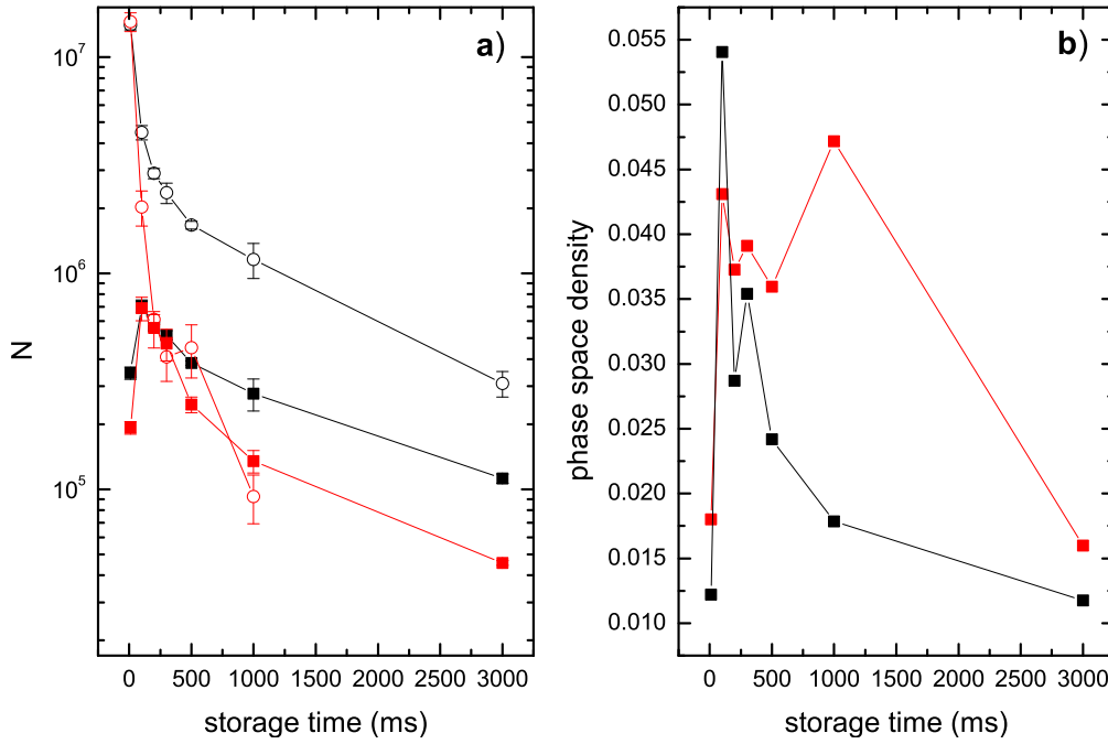
Figure 5.7: Number of atoms in the dimple (squares) and in the horizontal trap (circles) as a function of storage time for different power ratios a). The corresponding phase-space density is shown in b). For a power of 6.5 W in the horizontal trap and 3.5 W in the tilted trap (black lines) a partly compensation of the atoms lost from the dimple is observed due to a reloading from the horizontal trap. A continuous loading is prevented in the case of similar powers with 4.7 W in the horizontal and 5.2 W in the tilted trap (red lines). This results in a lower number of atoms and a higher phase-space density, since an heating effect from the continuously loaded atoms does not take place.
