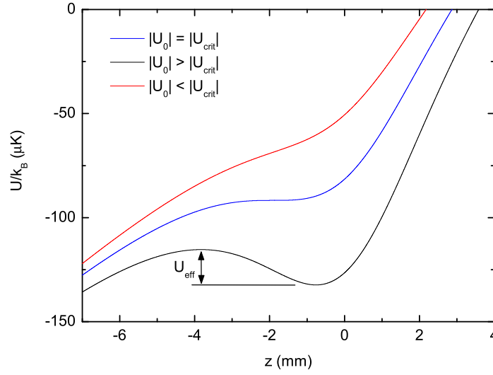
Figure 5.2: Potential in the tilted dipole trap for different optical powers. Only if the dipole potential |U_0| exceeds the critical value |U_{\text{crit}}| a local minimum in the potential appears and it becomes possible to trap atoms. The realized dipole trap has an effective depth of U_{\text{eff}} .
