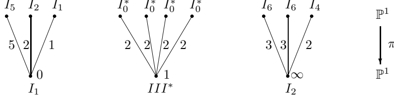
Figure III.33: A realization of [1,2,4,5,6,6]
