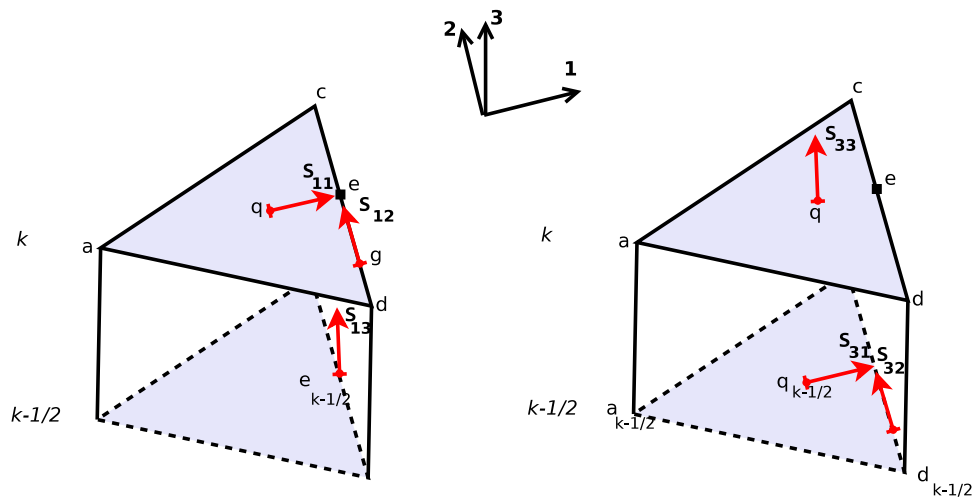
Figure 2. Schematic showing the locations at which the strain rates S_{ij} are defined for (left) horizontal and (right) vertical turbulent diffusion. The full and half vertical levels are indicated by k and k-1/2 , respectively, and the triangles at the half levels are marked by dashed line. Naming convention same as that of Figure 1 is used. The direction vectors are also indicated in the middle.
