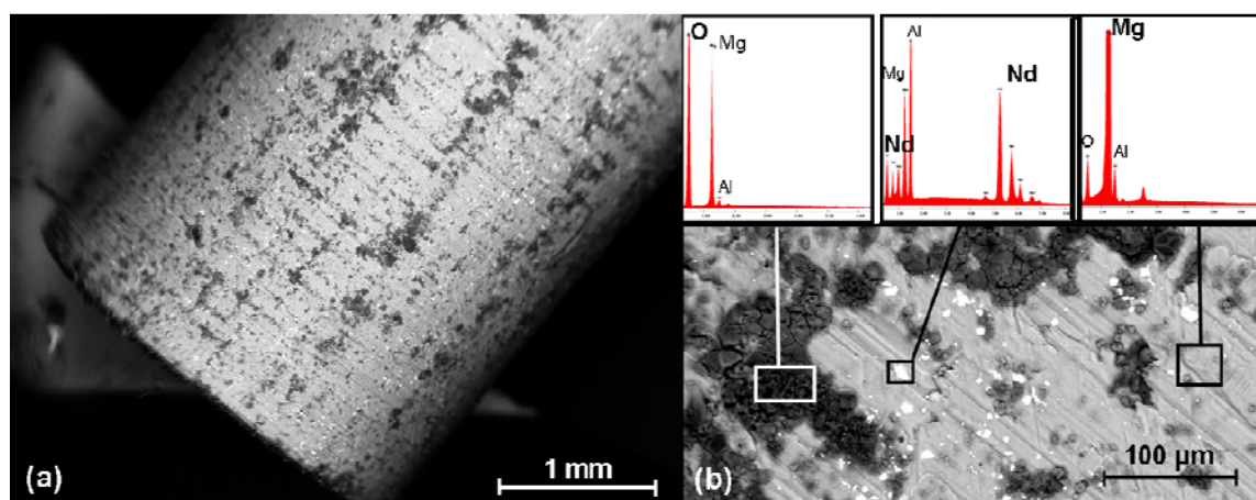
Figure 6. SEM images prior to implantation: (a) Overview of the pin's surface prior to the test; (b) EDX analysis of the pin's surface: preferentially detected Mg, Al, Nd and O. Each of the boxes mark the regions selected for the EDX analysis.
