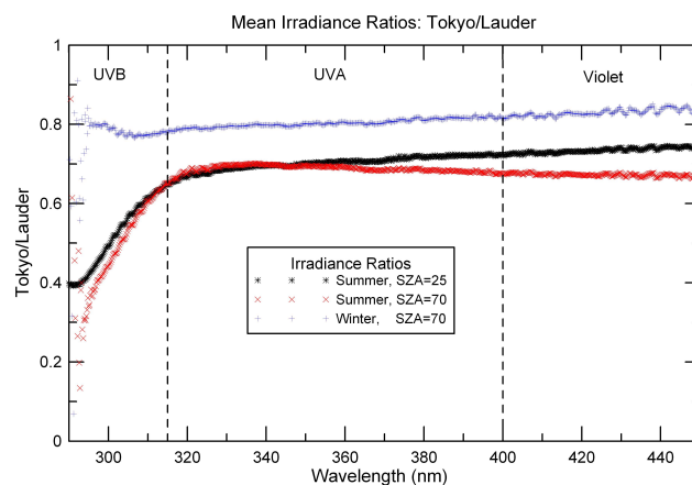
Fig. 3. Spectral ratios of Tokyo irradiances divided by Lauder irradiances for three conditions: summer, \text{SAZ}=25^\circ , and 70^\circ ; and winter \text{SAZ}=70^\circ .
