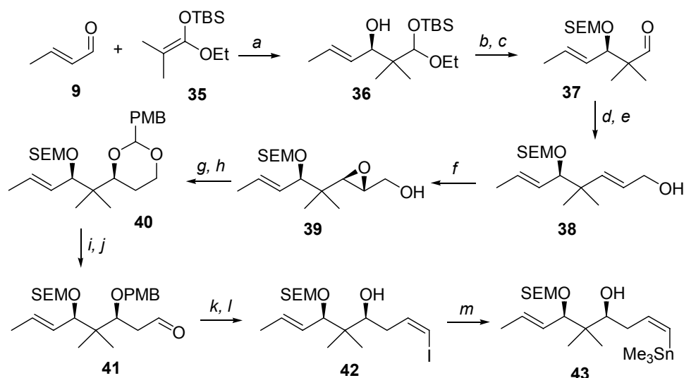
Abb. 14 Darstellung des C11-C19 Vinylstannans 43: (a) \text{BH}_3 \cdot \text{THF} , N -Tos- L -Valin, DCM, -78^\circ\text{C} , 73%; (b) SEMCl, i -Pr 2 EtN, DCM, -78^\circ\text{C} (c) AcOH, 79% über 2 Stufen; (d) (\text{EtO})_2\text{P}(\text{O})\text{CH}_2\text{CO}_2\text{Et} , NaH, PhMe, THF, > 95%; (e) DIBAH, DCM, -78^\circ\text{C} ; 76%; (f) D -(-)-DIPT, t -BuOOH, \text{Ti}(\text{i-PrO})_4 , DCM, -30^\circ\text{C} , 95%; (g) Red-Al, THF, -20^\circ\text{C} ; (h) p -Methoxybenzylidendimethylacetal, PPTS, DCM, 83% über 2 Stufen; (i) DIBAH, DCM, -78^\circ\text{C} , 92%; (j) DMP, Py, t -BuOH, DCM, 83%; (k) \text{IPh}_3\text{PCH}_2\text{I} , NaHMDS, HMPA, THF, -78^\circ\text{C} , 67%; (l) DDQ, DCM, \text{H}_2\text{O} , 79%; (m) \text{PdCl}_2(\text{PPh}_3)_2 , (\text{Me}_3\text{Sn})_2 , \text{Li}_2\text{CO}_3 , THF, RT, 74%.
