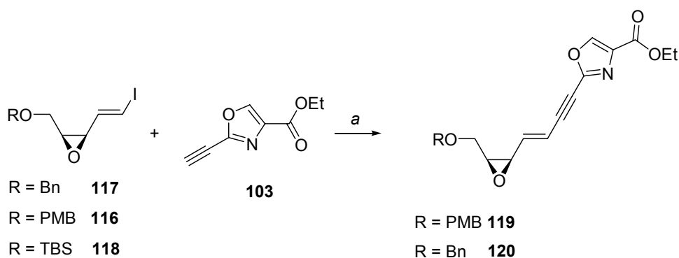
Abb. 57 Sonogashira Kupplung zum unnatürlichen C1-C11 Epoxyoxazol: (a) PdCl 2 (PPh 3 ) 2 , Et 3 N, DMF, RT, 8 h, 14% (R = PMB), 10% (R = Bn), 0% (R = TBS).
