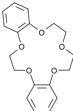
Dibenzo-15-Krone-5
