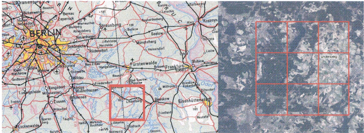
FIG. 2. Location of the experimental area roughly 65 km southeast of Berlin. (right) The Landsat picture (copyright GEOSPACE Herold, 1997 Herold Business Data AG/GEOSPACE Beckel Satellitenbilddaten GmbH) gives an impression of the landscape heterogeneity inside nine grid cells of the weather forecast model of DWD (LM). Each grid cell covers an area of 7 km × 7 km. The western part is dominated by forested areas and the eastern part by farmland.
