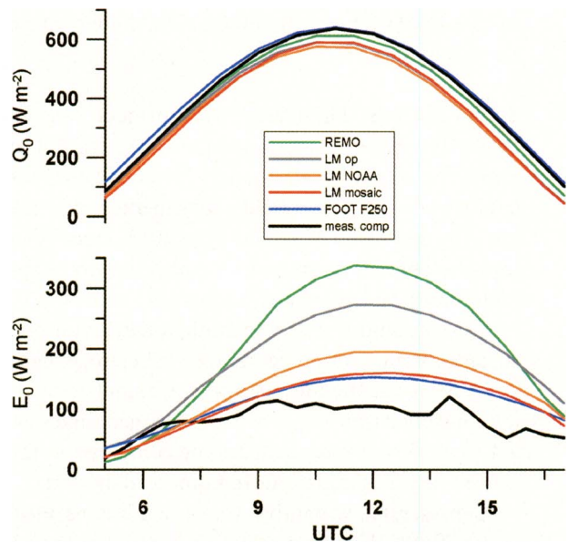
FIG. 10. Diurnal cycle of (top) Q_0 and (bottom) E_0 computed by different mesoscale models for the whole LITFASS area for 30 May 2003: REMO (18-km resolution), different LM versions (7-km resolution), FOOT3DK (250-m resolution), and area-averaged flux composite from the surface stations. The curves for the LM denote three different model runs: LM op is the operational run, LM NOAA uses LAI and vegetation cover derived from AVHRR, LM mosaic uses the mosaic method with 1-km resolution of the surface parameters.
