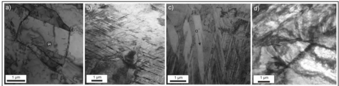
Fig. 2. TEM bright field images of a) the as-received X40MnCrAl19-2 and after deformation to b) 50 % at RT, c) 45 % at -196 °C and d) 35 % at 400 °C.
