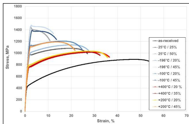
Fig. 1. Monotonic stress-strain curves of the X40MnCrAl19-2 steel following different pre-treatments (partly recomputed from [6]).
