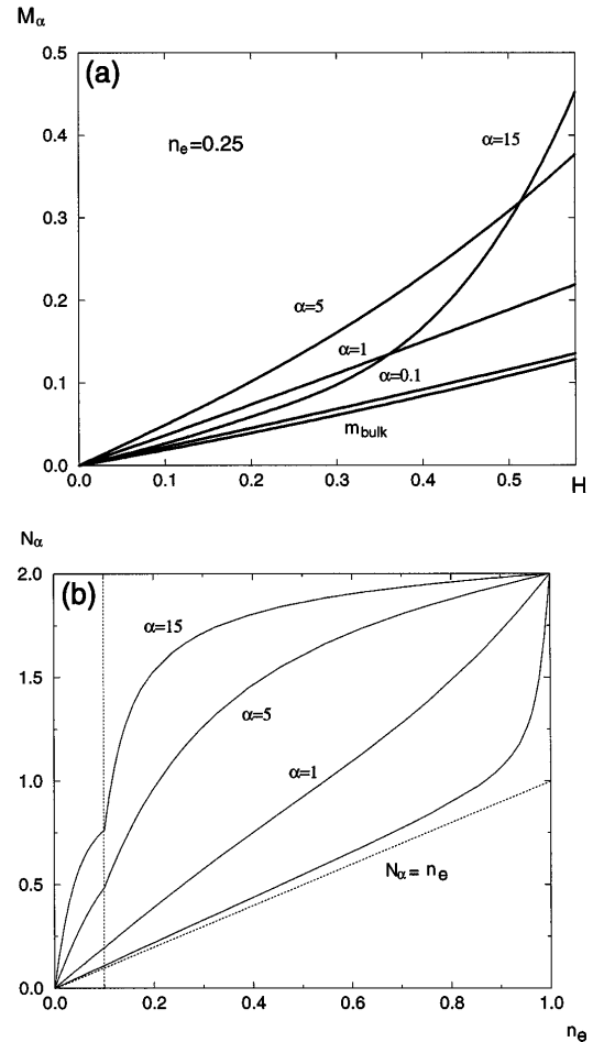
FIG. 2. (a) Impurity magnetization as a function of magnetic field for band filling n_e = 0.25 and several values of \alpha . (b) Number of electrons located at the impurity as a function of the bulk electron density for fixed magnetic field H = 0.1 and several values of \alpha . The dotted line denotes the critical electron density n_c below which the ground state is ferromagnetic.
