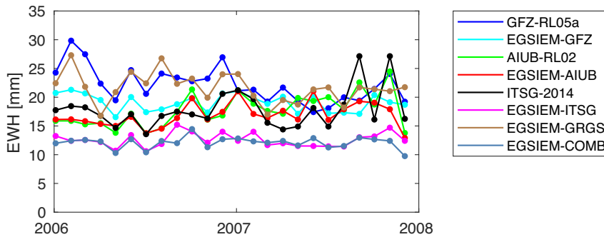
Figure 5. Weighted RMS over the oceans of filtered monthly solutions of the EGSiEM ACs and of the combined monthly solutions.
