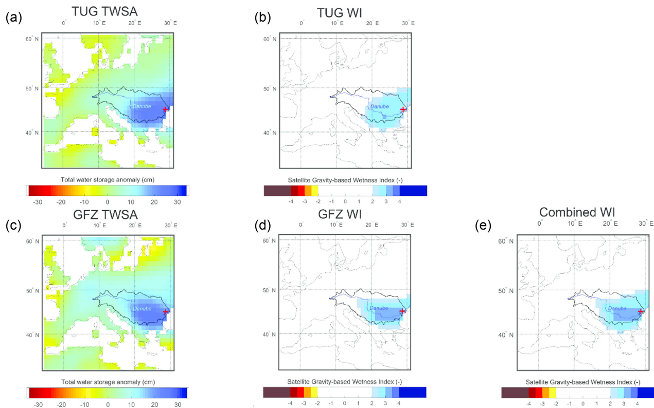
Figure 13. Daily gravity-based total water storage anomalies (TWSA) and gravity-based Wetness Indices (WI) for the Danube basin for 2006 April 26 based on TUG gravity solution (a, b), GFZ gravity solution (c,d) as well as the combined WI (e). The red cross indicates the location of the gauging station Ceatal Izmail.
