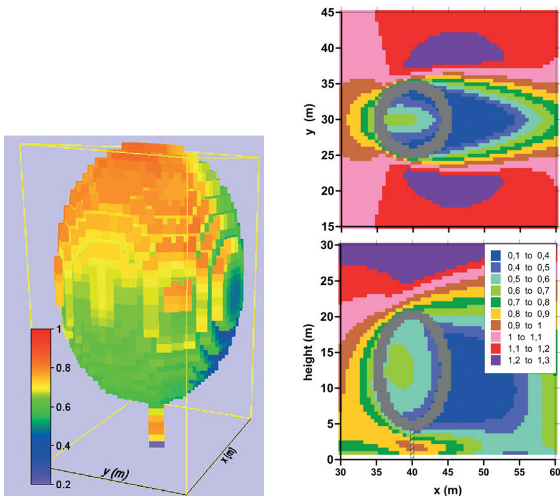
Figure 2: Mean wind speed normalized with the undisturbed 10m value. Left: three dimensional distribution above the tree surface. Right above: horizontal cross section at a height of 12 m (middle of the crown) Right below: vertical cross section along the centre. Grey areas indicate leaf area.
