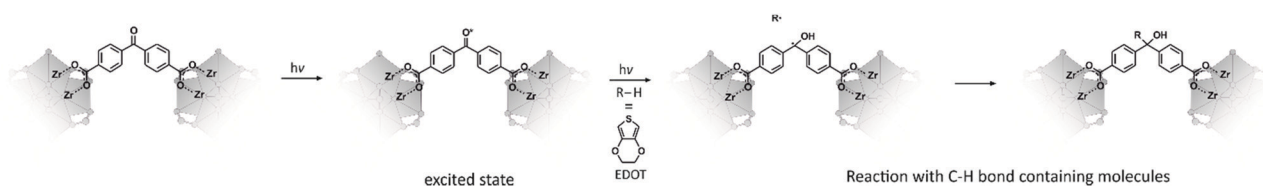
Scheme 2 Schematic mechanism for the photoreaction of the keto group of benzophenone units in the framework of Zr-bzpdC-MOF: formation of a ketyl radical which then reacts with a C–H bond-containing molecule (in this study EDOT), resulting in a covalent bond.
