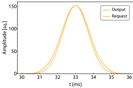
(c) Field response in z -direction.
