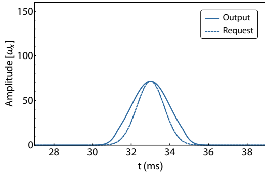
(a) Field response in x -direction.
