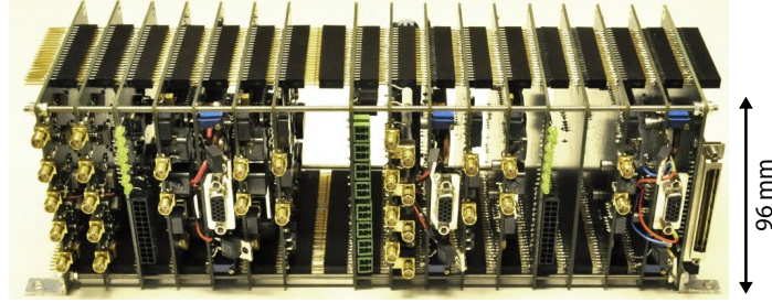
Figure 17: Picture of the assembled T-Bus stack prior to integration. The single stack holds 6 laser current drivers, 4 TA current drivers, 6 temperature controllers, 2 DDS-based AOM controllers with 4 channels each, a frequency controller to stabilize 4 lasers and a shutter driver with 8 channels. The total power consumption amounts to approximately 122 W.
