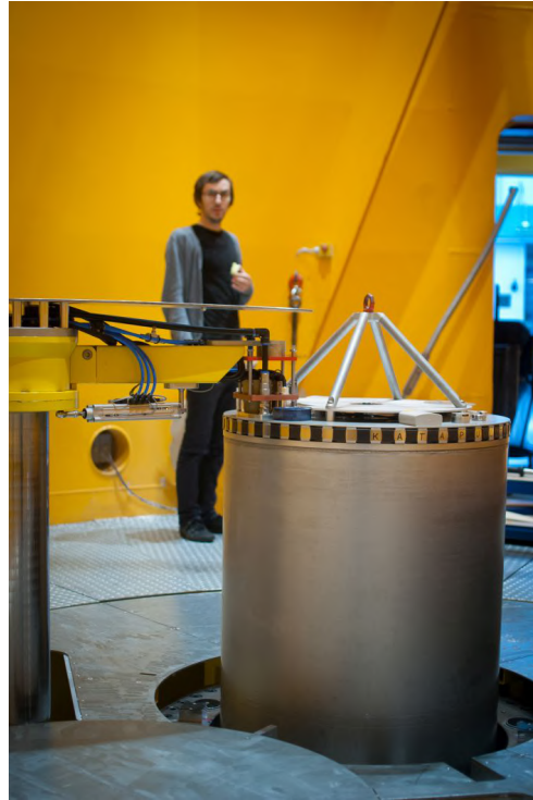
Figure 37: The capsule sits in the catapult receptacle and is docked with the supply arm prior to evacuation of the tower. Once the setup is retracted to launch position 9 m below the drop tube, the scientist have a 5 min launch window before the process is aborted.
