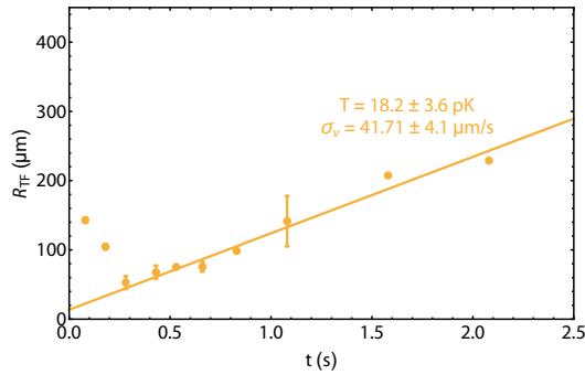
(a) Linear fits to x' lens data.
