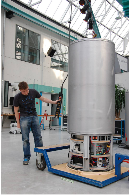
Figure 32: Capsule hull is lowered onto the capsule for the first pre-test. The two visible platforms at the bottom constitute the capsule base structure. The lowest level holds most of the systems batteries. The next platform houses the secondary capsule control computer in charge of communication to the control room.
