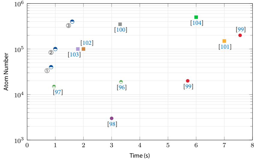
Figure 29: Comparison of the fastest BEC machines. Circles mark atom chip based experiments [96–99], squares indicate experiments using dipole traps [100–104]. Ref. [102] describes a ^{84}\text{Sr} experiment. Ref. [103] marks a recent dipole trap setup using ^{174}\text{Yb} . Ref. [104] is a hybrid apparatus using a magnetic quadrupole trap and a dipole trap to evaporatively cool metastable ^4\text{He} . All other experiments use ^{87}\text{Rb} . Semi-filled symbols mark compact and transportable setups. The performance of the QUANTUS-2 apparatus is represented by three cases, ① – ③.
