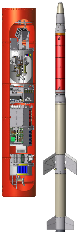
Figure 97: CAD drawing of the MAIUS-1 mission payload and its sounding rocket platform [110].
