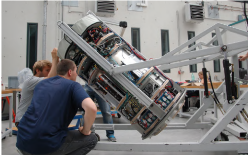
(a) The capsule being rotated around a horizontal axis using a hydraulic crane.
