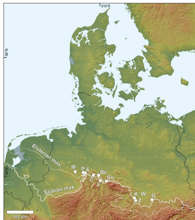
Figure 10. Location of the study area in northern Germany, showing the maximum extent of the Middle Pleistocene Elsterian and Saalian ice sheets in Central Europe and associated ice-marginal delta systems (Adopted from Reference [51]). Notation used for deltas is as follows: Be Betheln delta, Bo Bornhausen delta, C Coppenbrügge subaqueous fan and delta complex, E Emme delta, F Freden delta, G Großsteinberg delta, K Karsdorf delta, M Markendorf delta, P Porta subaqueous fan and delta complex, W Wünsch delta, Z Zeuchfeld delta.
