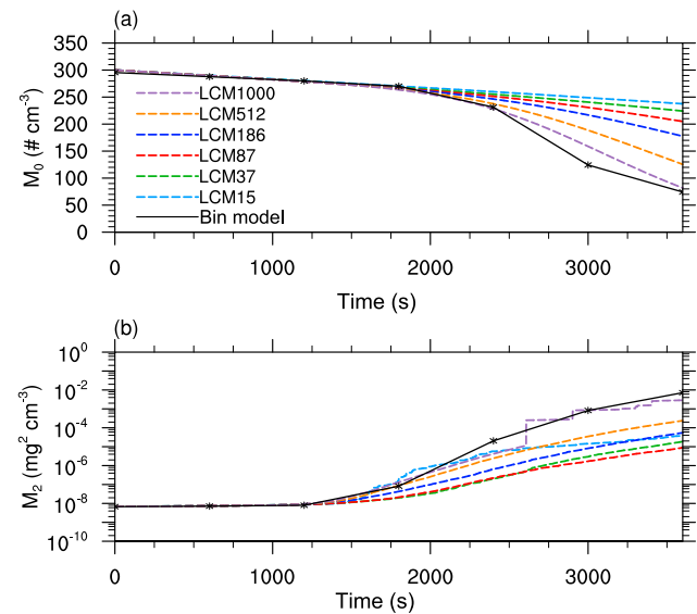
Figure 4. Moments of the mass density distribution as a function of time obtained from the single-box simulations. The black solid line denotes the solution of Wang et al. (2007). The colored dashed curves show the solution of the LCM with different numbers of superdroplets per grid box.
