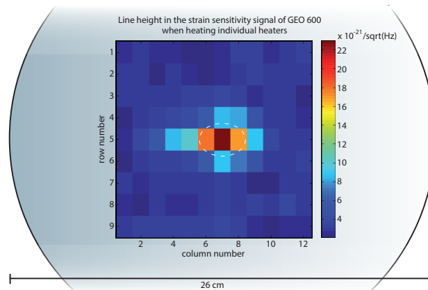
Fig. 3. Measured overlap of the projected pixels of the heater array and the fundamental TEM_{00} mode of the main laser beam in GEO 600. For comparison, the ( 1/e^2 in intensity) size of the laser beam spot on the beam splitter is represented via white dashes, while the outline of the beam splitter is depicted in the background.
