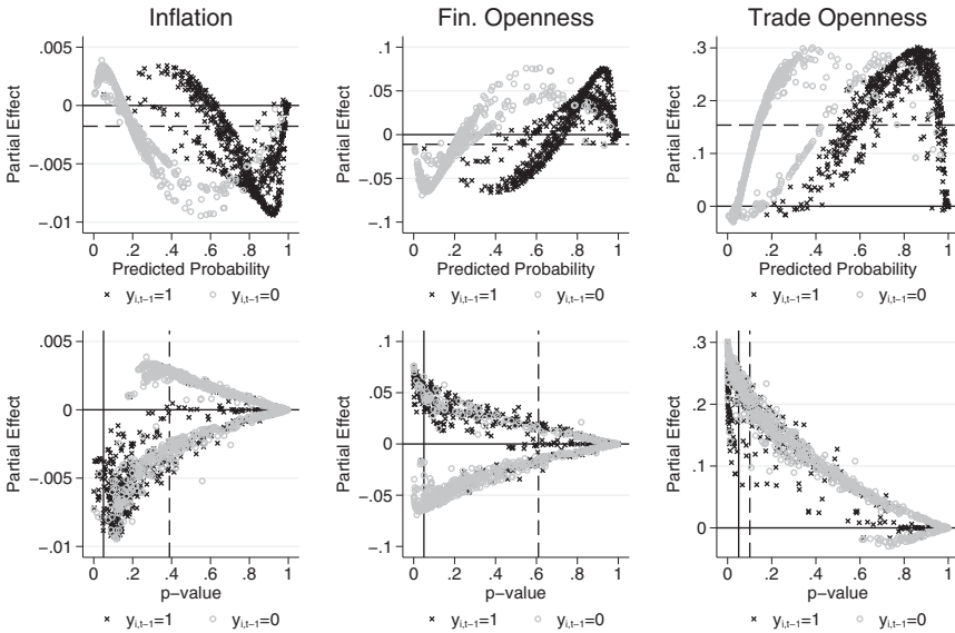
FIGURE 2. Partial effects of interaction terms in logit model. The dashed line refers to the APE in the upper panel and the p -value of a Wald test that the APE is zero in the lower panel. “Predicted probability” is the probability of stagnation, P(y_{it} = 1) .
