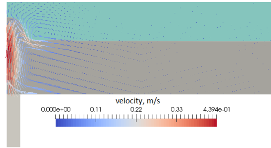
Fig. 9: Example velocity and surface deformation, h_0=20mm, I_{rms}=1kA
