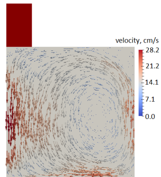
Fig. 5: Example velocity distribution, I=1kA
