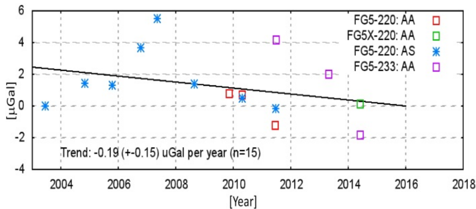
Figure 4: Gravity variations at Onsala as obtained with the FG5 gravimeters of LM and LUH, after applying reductions from SCG GWR#54 (available since 2009).
