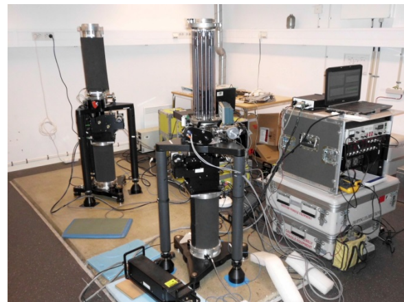
Figure 3: OSO absolute gravity site with the absolute gravimeter FG5X-220 (point AA, room center) of LUH and FG5-233 (AC) of LM.
