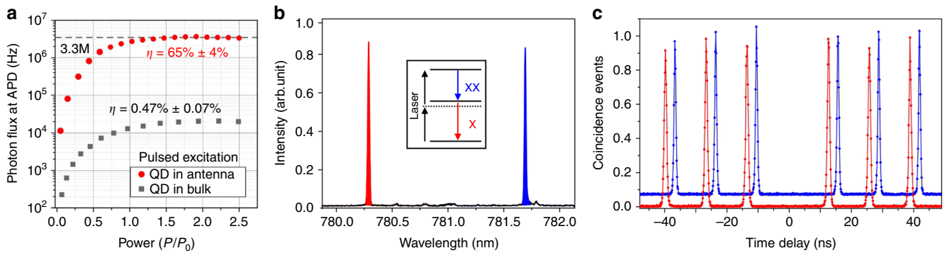
Fig. 2 Characterization of the broadband dielectric antenna and resonant excitation of XX state under 76 MHz pulsed excitation. a Single photon flux measured on APD, plotted as a function of laser excitation power (in saturation units), for a QD in dielectric antenna (red dot symbol) and in unprocessed bulk substrate (gray square symbol). At saturation, 3.3 million of single photons per second are detected. b Resonant excitation of the XX state using a two-photon pump scheme. The residual laser signal is strongly suppressed by the setup. c Intensity-correlation histogram from the X transition under two photon pumping excitation. Nearly ideal single-photon emissions is demonstrated by the vanishing multi-photon events at zero time delay g^2(0) \cong 0.002 for both X and XX photons
