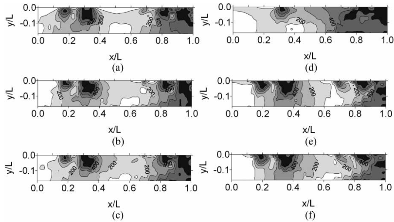
Fig. 9 Subsurface von Mises stress contours of the thermal elasto-plastic contact of the rough surface subject to different frictional heat inputs, E_T = 0.0 (unit: MPa): (a) f\bar{v} = 0.0\text{m/s} , f = 0.0 ; (b) f\bar{v} = 0.1\text{m/s} , f = 0.2 ; (c) f\bar{v} = 0.2\text{m/s} , f = 0.2 ; (d) f\bar{v} = 0.5\text{m/s} , f = 0.2 ; (e) f\bar{v} = 0.1\text{m/s} , f = 0.5 ; and (f) f\bar{v} = 0.2\text{m/s} , f = 0.5
