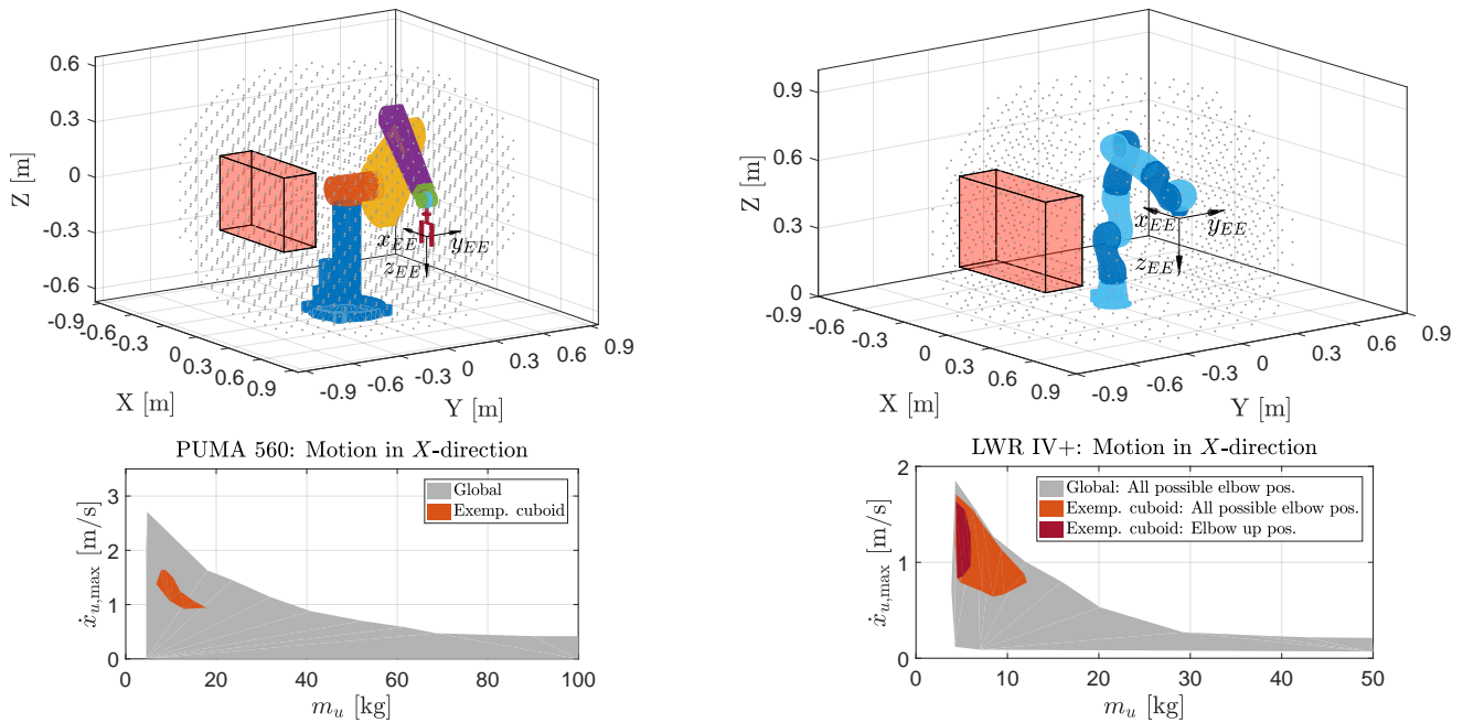
Fig. 4. Map representation of the PUMA 560 and the LWR IV+ for motions in Cartesian X -direction. In the upper row, the feasible Cartesian positions for the considered end-effector orientation are illustrated as dots, an exemplary subset of the workspace, a cuboid with 60 \times 20 \times 40 cm, is colored red. In the lower row, the mass/velocity representations of the PUMA 560 and LWR IV+ are depicted.
