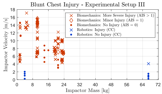
Fig. 3. Summary of relation between mass, velocity, and injury for selected data on the chest [11]–[13].
