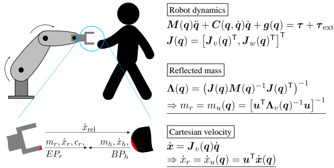
Fig. 2. Collision model for representing the instantaneous dynamic properties of the impactor/robot and subject/human. In the robot dynamic equations, \mathbf{q} \in \mathbb{R}^n denotes the generalized coordinates, \mathbf{M}(\mathbf{q}) \in \mathbb{R}^{n \times n} the symmetric, positive definite mass matrix, \mathbf{C}(\mathbf{q}, \dot{\mathbf{q}}) \in \mathbb{R}^{n \times n} the Coriolis and centrifugal matrix, and \mathbf{g}(\mathbf{q}) \in \mathbb{R}^n the gravity torque vector. The motor joint torque is denoted \boldsymbol{\tau} \in \mathbb{R}^n and the external joint torques \boldsymbol{\tau}_{\text{ext}} \in \mathbb{R}^n . The Jacobian matrix associated with the impact location is \mathbf{J}(\mathbf{q}) \in \mathbb{R}^{6 \times n} and the Cartesian mass matrix is \boldsymbol{\Lambda}(\mathbf{q}) \in \mathbb{R}^{6 \times 6} . The scalar mass and velocity in normalized Cartesian direction \mathbf{u} \in \mathbb{R}^3 are denoted m_u(\mathbf{q}) \in \mathbb{R} and \dot{x}_u(\mathbf{q}) \in \mathbb{R} .
