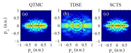
Figure 1. Vectorial momentum distributions for the H atom ionized by a laser pulse with a duration of n = 8 cycles, wavelength of \lambda = 800 nm, and peak intensity of I = 9 \times 10^{13} W/cm 2 obtained from (a) the QTMC model, (b) solution of the TDSE, and (c) the present SCTS model. The laser field is linearly polarized along the z-axis.
