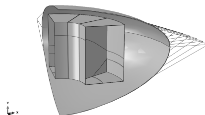
Figure 2: Model of a quarter of the capsule and the 'steering-wheel' cutting geometry
