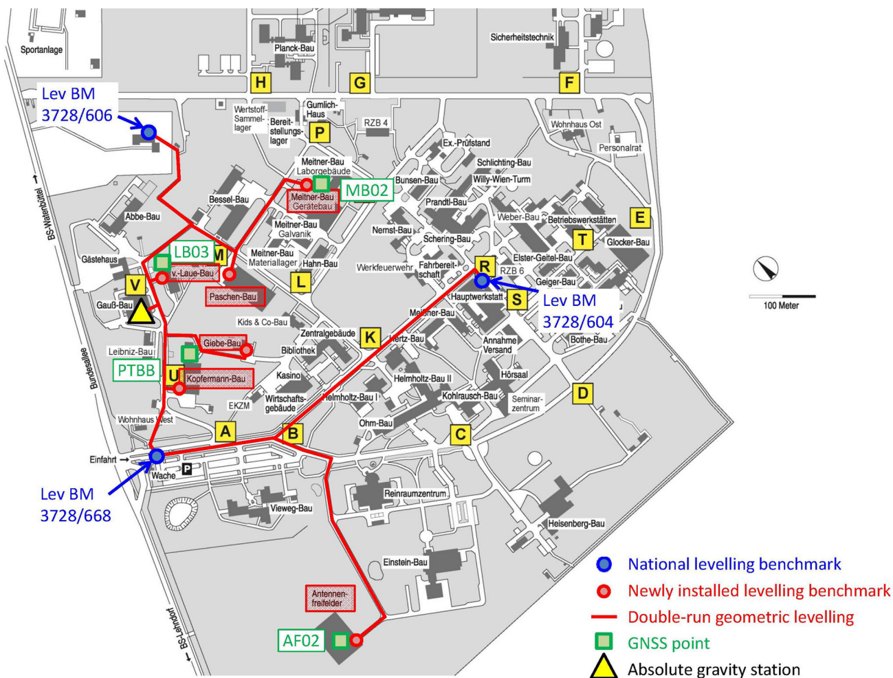
Fig. 2 Levelling benchmarks and lines, GNSS stations, and an absolute gravity point at PTB
