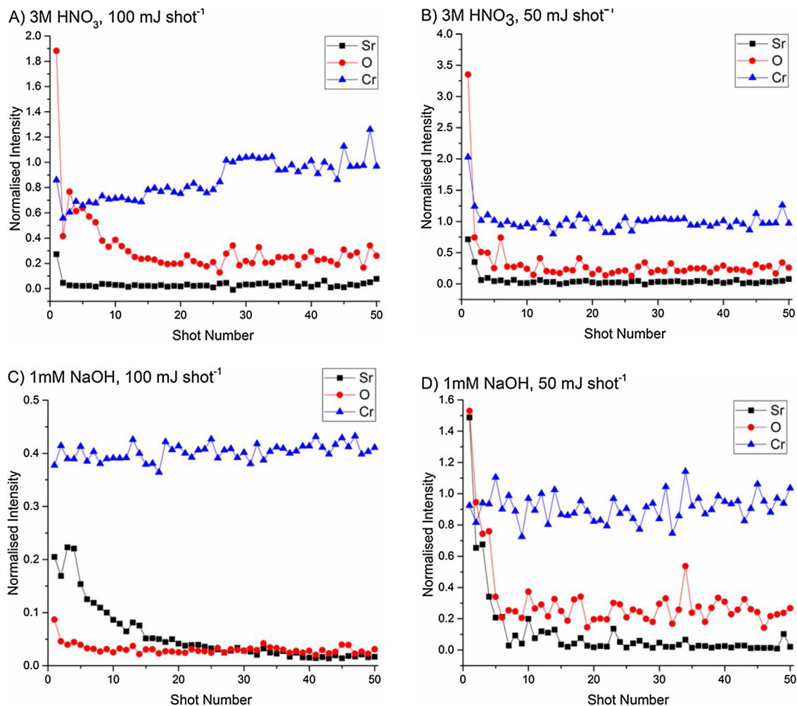
Fig. 3. Comparison of LIBS depth profiles measured in an argon environment for acidic and alkaline contaminated stainless steel at 100 mJ and 50 mJ laser energy. The Sr signal in (C) was scaled by a factor of 0.1 for clarity.
