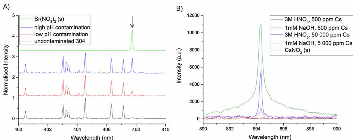
Fig. 2. Comparison of LIBS emission spectra in the regions of interest for (A) Sr, and (B) Cs detection. The arrow shows the position of the Sr II 407.77 nm line. Measurement was performed under open air conditions at a laser output energy of 100 mJ. The spectra in (A) were normalised to 1 for ease of comparison.
