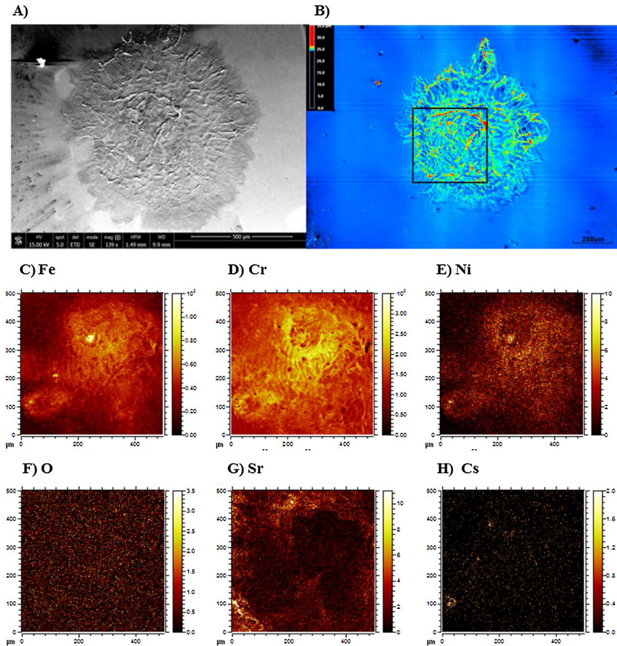
Fig. 6. (A) SEM morphology and (B) confocal microscopy analysis of a crater formed on an alkaline contaminated steel sample from a single 100 mJ laser shot under an argon atmosphere. TOF-SIMS elemental analysis of the highlighted region in (B) for the elements (C) Fe, (D) Cr, (E) Ni, (F) O, (G) Sr, and (H) Cs.
