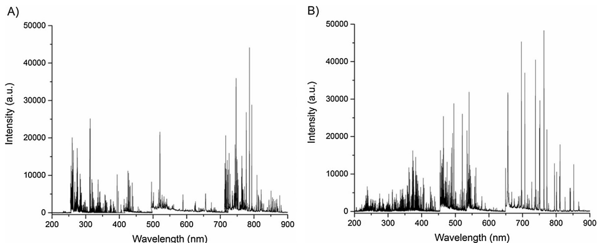
Fig. 1. LIBS emission spectra for 'as received' AISI Type 304 stainless steel under air (A) and argon (B) atmospheres.
