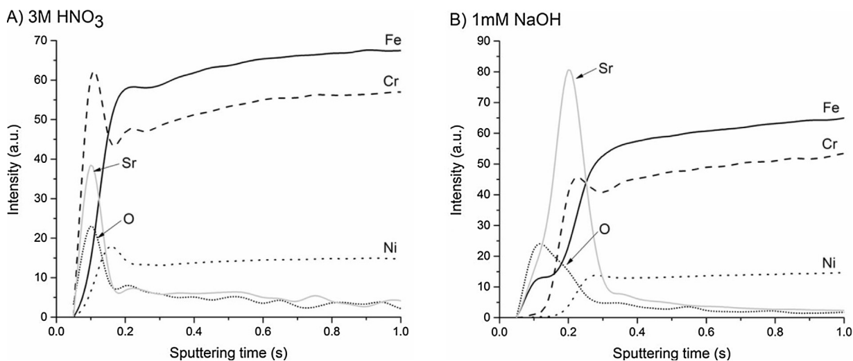
Fig. 4. GD-OES depth profiles of 304 stainless steel contaminated in 3 M HNO 3 and 1 mM NaOH. For clarity the Sr signals have been scaled by a factor of 100 for the acidic and alkaline systems.
