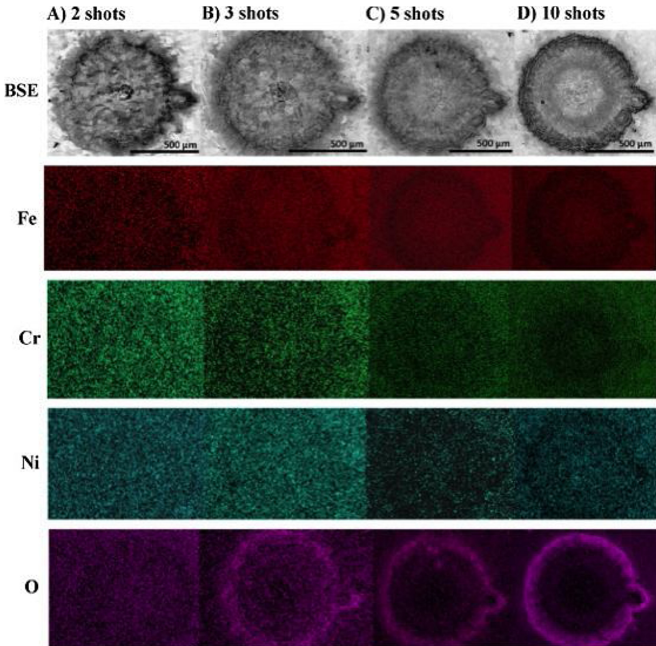
Fig. 5. SEM image and SEM-EDX elemental maps of LIBS craters formed on the high pH contaminated steel surface after a different number of 100 mJ shots under argon.
