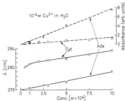
Fig. 4. Plot of the UV CT-absorption band (wavelength and intensity) vs the concentration of adenine ( \lambda : \times , OD: +) and cytosine ( \lambda : \circ , OD: \square ).
