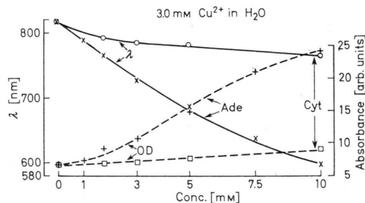
Fig. 5. Plot of the visible CT-absorption band (wavelength and intensity) vs the concentration of adenine ( \lambda : \times , OD: +) and cytosine ( \lambda : \circ , OD: \square ).
