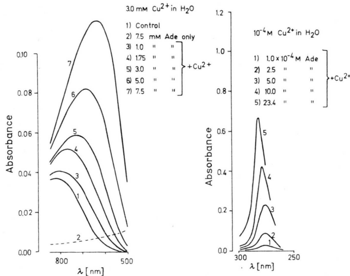
Fig. 3. Difference spectra of adenine and mixture of \text{Cu}^{2+} and adenine in an aqueous solution.
