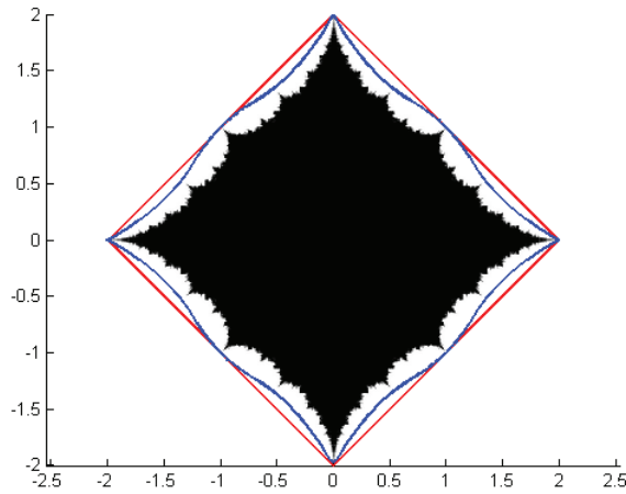
Figure 1. The boundary of \sqrt{N(A^2)} (blue), the boundary of N(A) (red) and a lower bound to \text{sp}(A) consisting of spectra of periodic operators and the closed unit disk (black, see [2] and [3]) in the case \sigma = 1 .
