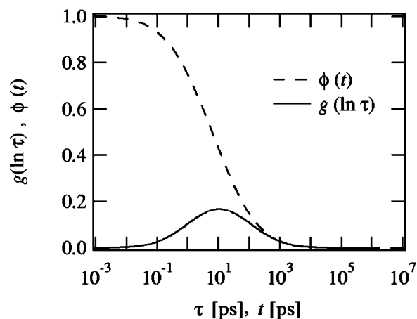
FIG. 10. Log-normal distribution of correlation times g(\ln \tau) and the resulting dynamic function \phi(t) as obtained by fitting Eqs. (2), (6), and (5) to the S(Q,t) data, shown exemplarily for \text{Ca}_{0.5}\text{AlSi}_3\text{O}_8 \cdot 1.3\text{H}_2\text{O} (AQ8) at 321 K, Q=1.85 \text{ \AA}^{-1} .
