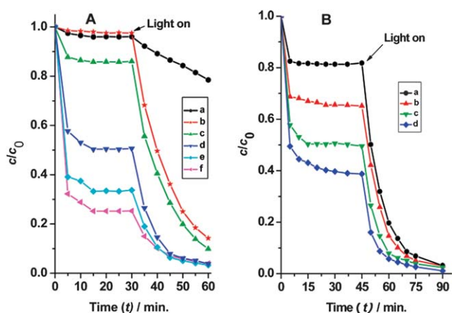
Fig. 11 Photocatalytic degradation of RhB monitored as the normalized concentration change versus irradiation time in the presence of (A) mesoporous \text{TiO}_2 - \text{SiO}_2 composites prepared with different Ti/Si ratios. (a) Mesoporous \text{TiO}_2 calcined at 400^\circ\text{C} for 2 h; (b) commercial photocatalyst P25; (c) mesoporous 90\text{TiO}_2 - 10\text{SiO}_2 composite calcined at 700^\circ\text{C} for 2 h; (d) mesoporous 80\text{TiO}_2 - 20\text{SiO}_2 , (e) 70\text{TiO}_2 - 30\text{SiO}_2 , and (f) 60\text{TiO}_2 - 40\text{SiO}_2 composites calcined at 850^\circ\text{C} for 2 h. (B) Photocatalytic degradation for mesoporous 80\text{TiO}_2 - 20\text{SiO}_2 composites calcined at 700^\circ\text{C} for 4 h (a), 800^\circ\text{C} for 2 h (b), 850^\circ\text{C} for 2 h (c), and 900^\circ\text{C} for 2 h (d). Reprinted with permission from ref. 92, Copyright 2007 ACS.
