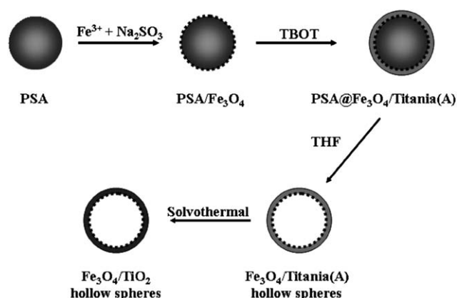
Fig. 8 Schematic procedure used for fabrication of magnetic TiO 2 hollow spheres (A: amorphous). Reprinted with permission from ref. 64, Copyright 2009 ACS.
