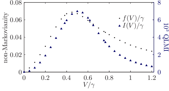
FIG. 4. Non-Markovianity f(V) and the QLMI I(V) of the steady state for different values of the interaction strength V ( \Omega = \gamma ).
