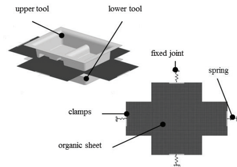
Fig. 2 Simulation model in LS-Dyna
