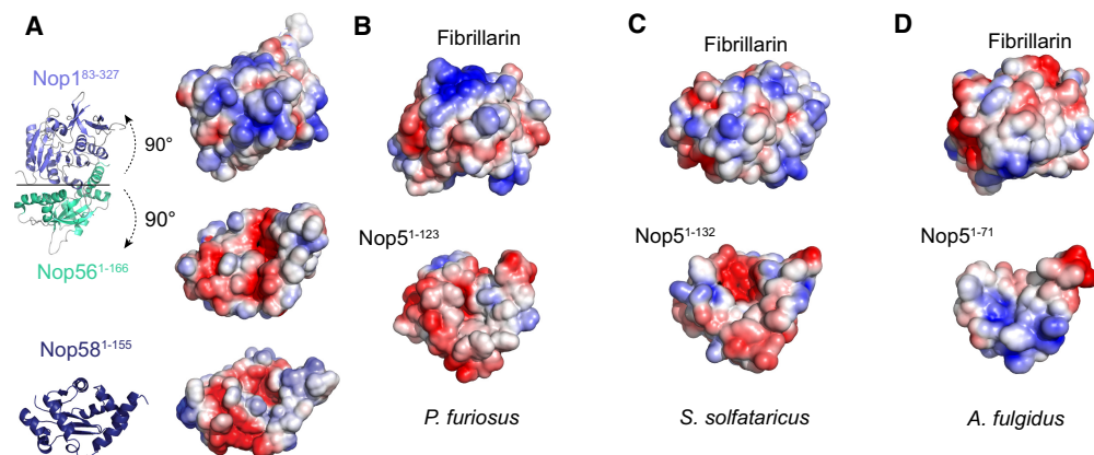
FIGURE 5. Comparison of the solvent-accessible surface electrostatics at the protein–protein interface in archaeal and eukaryotic complexes. (A) Sc Nop56 1–166 –Nop1 83–327 complex; (B) Pf Nop5 1–123 –Fibrillarlin (PDB-ID: 2NNW); (C) Ss Nop5 1–132 –Fibrillarlin (PDB-ID: 3ID5); (D) Af Nop5 1–71 –Fibrillarlin (PDB-ID:1NT2). Blue, red, and white represent positive, negative, and neutral charges, respectively.
