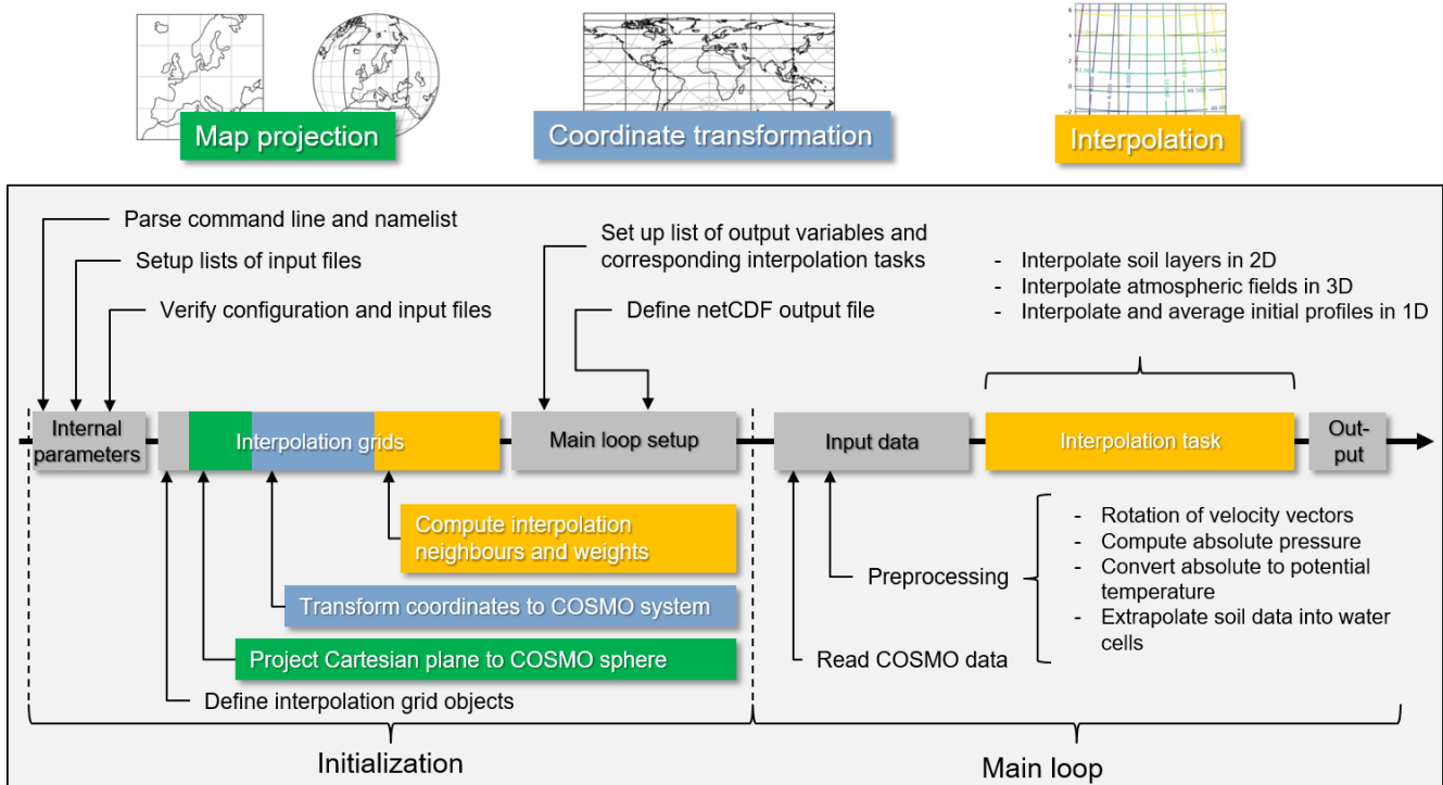
Figure 6. Diagram of INIFOR’s program flow.
