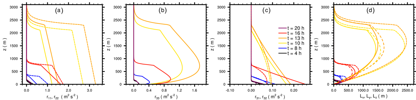
Figure 13. Parameterized components of the Reynolds-stress tensor as well as turbulent length scales at different points in time. In panels (a) and (c), the solid (dashed) line belongs to r_{11} ( r_{22} ) and r_{31} ( r_{32} ), respectively. In panel (d) the solid, fine, and coarse dashed lines belong to L_x , L_y , and L_z , respectively.
