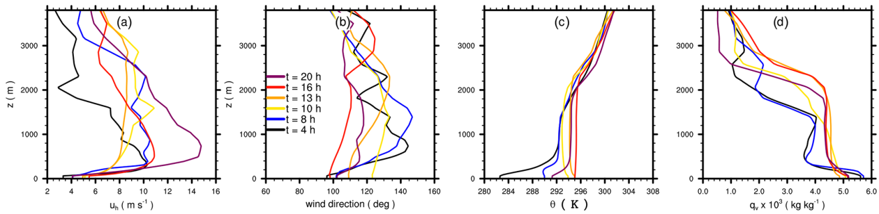
Figure 7. COSMO-derived vertical profiles of (a) horizontal wind speed, (b) mean-wind direction, (c) potential temperature, and (d) specific humidity prescribed at the lateral domain boundaries at different points in time after the start of the simulation at 00:00 UTC.
