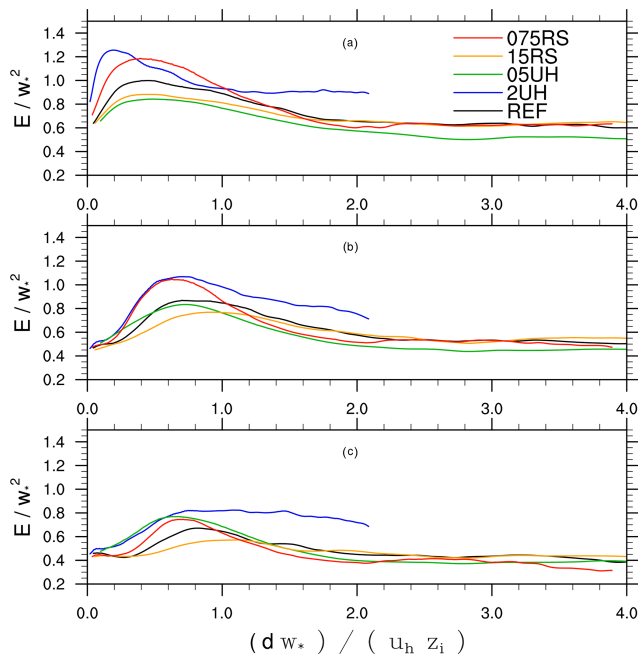
Figure 17. Horizontal profile of 30 min time-averaged resolved-scale TKE on 13:00 UTC depending on the normalized distance to the inflow boundary at (a) 0.1 z_i , (b) 0.5 z_i , and (c) 0.75 z_i .
