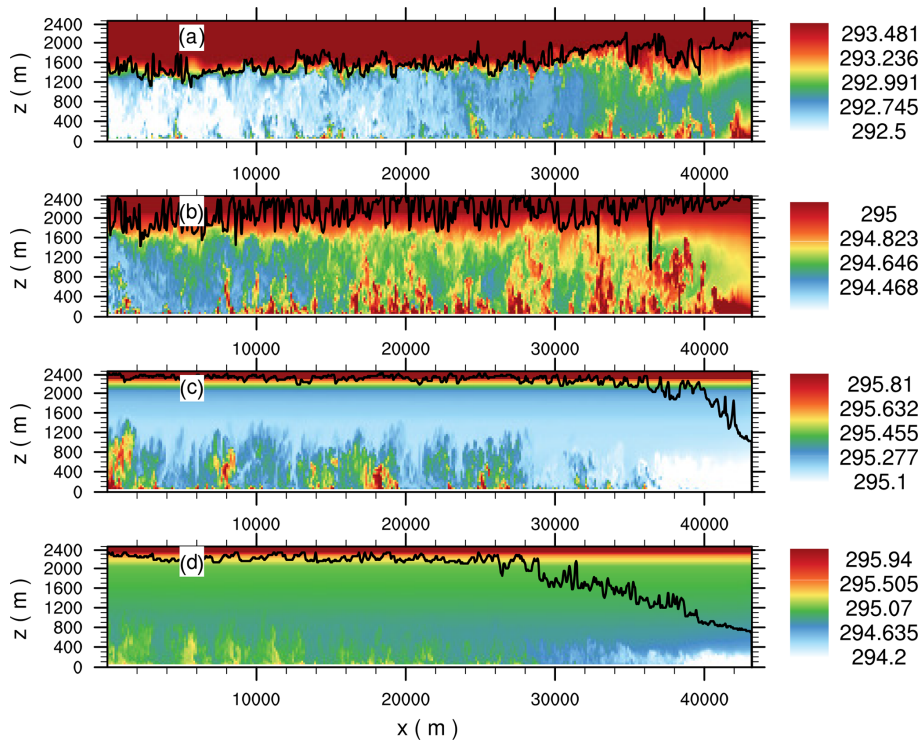
Figure 11. Instantaneous x – z cross-section of the simulated potential temperature (contours) and local boundary-layer height (black solid line) in PALM at (a) 10:00 UTC, (b) 13:00 UTC, (c) 16:00 UTC, and (d) 16:30 UTC. The boundary-layer height is calculated according to the Richardson bulk criterion. The inflow boundary is on the right. Please note that the inflow direction is from the south-east, meaning that the x axis does not correspond with the distance to the inflow boundary. The cross-section is taken at y = 32\,200 m (indicated by the dashed black line in Fig. 12b) where the potential temperature is not affected by advection from the southern inflow boundary. Also note the different contour levels and colour bars in each panel, which we set to emphasize the horizontal heterogeneity of the simulated boundary layer at the different times of the day.
