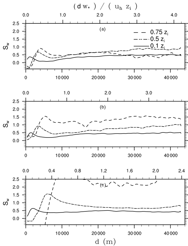
Figure 15. Horizontal profiles of 30 min time-averaged skewness S_w of w depending on the distance to the inflow boundary. S_w is shown for the lower, middle, and upper parts of the boundary layer at (a) 10:00 UTC, (b) 13:00 UTC, and (c) 16:00 UTC. The lower abscissa indicates the absolute distance to the inflow boundary, while the upper abscissa indicates the travel time of an imposed signal normalized with the eddy-turnover time. S_w is averaged over similar distances to the inflow boundary.
