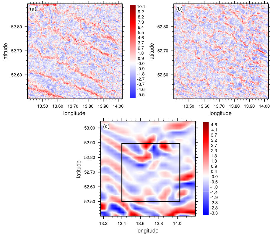
Figure 18. Horizontal cross-sections of the instantaneous vertical velocity component ( \text{m s}^{-1} ) at 12:00 UTC at z = 500 \text{ m} from (a) a PALM simulation with heterogeneous lateral and top boundary values given ( \text{LOD} = 2 ), (b) a PALM simulation with homogeneous boundary values given ( \text{LOD} = 1 ), and (c) a COSMO simulation. The black box in panel (c) indicates the location of the nested PALM domain within COSMO. The horizontal grid spacing in COSMO is 0.025^\circ . Please note that, for sake of comparison, the PALM axes are plotted in ( ^\circ ) as well, even though PALM uses Cartesian coordinates.
