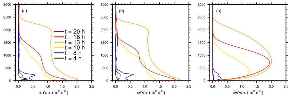
Figure 8. Variances of the velocity components: (a) for the u component, (b) for the v component, and (c) for the w component. The variance is computed from the region where the turbulent flow has been already adjusted.
