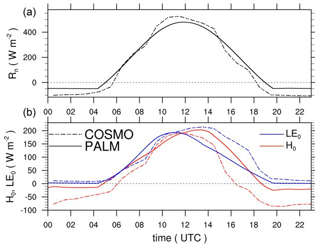
Figure 10. Time series of surface net radiation (a) and surface latent and sensible heat flux (b) from COSMO (dashed) and PALM (solid). Values are horizontally averaged over the corresponding domain. The fine horizontal dashed line indicates zero surface net radiation and heat fluxes, respectively. Please note the different temporal resolution between PALM and COSMO, with COSMO values only defined hourly.
