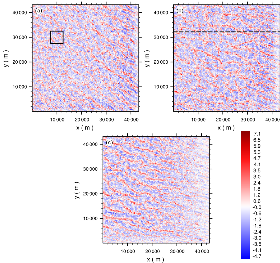
Figure 12. Horizontal cross-sections of the instantaneous vertical velocity component at z = 500 m for (a) 10:00 UTC, (b) 13:00 UTC, and (c) 16:00 UTC, with mean wind blowing from the south-east. The black box in panel (a) indicates the inner domain used to average the profiles shown in Fig. 9, while the dashed black line in panel (b) indicates the location of the x - z cross-section shown in Fig. 11.
