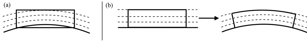
Figure 4. Schematic comparison of direct spherical-to-Cartesian transformation (a) and the inverse plate carrée projection (b). The schematic shows a vertical cut through the atmosphere and Earth’s surface (solid arc). The solid boxes represent the PALM domain and dashed arcs indicate isosurfaces of Earth’s gravitational potential.
