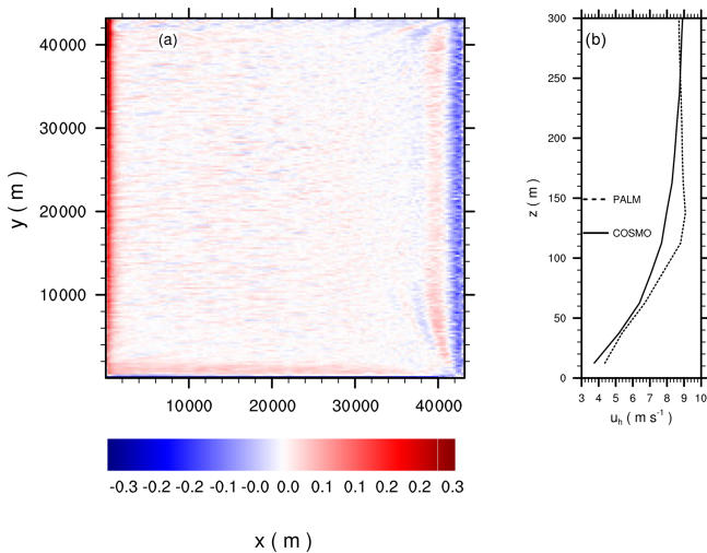
Figure 19. Horizontal cross-section of 30 min time-averaged (a) vertical velocity component at 03:00 UTC at z = 100 m. In addition, panel (b) shows corresponding vertical profiles of the horizontal wind speed averaged over a 10 \times 10 km area located at the domain centre, as well as the lateral inflow profile from the COSMO solution. The wind blows from the east.
