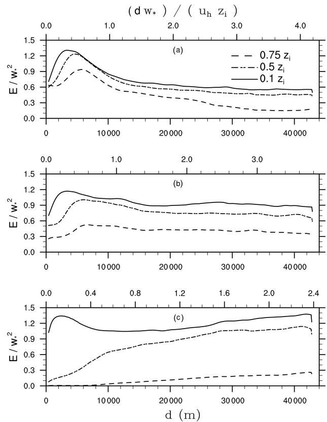
Figure 14. Horizontal profiles of 30 min time-averaged resolved-scale TKE depending on the distance to the inflow boundary. The TKE is shown for the lower, middle, and upper parts of the boundary layer at (a) 10:00 UTC, (b) 13:00 UTC, and (c) 16:00 UTC. The lower abscissa indicates the absolute distance to the inflow boundary, while the upper abscissa indicates the travel time of an imposed signal normalized with the eddy-turnover time. The TKE is averaged over similar distances to the inflow boundary.
