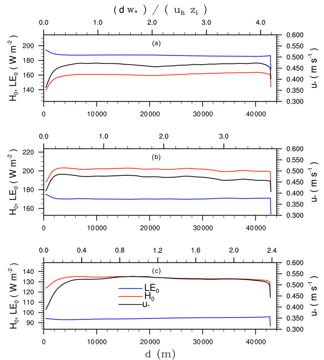
Figure 16. Horizontal profiles of 30 min surface latent LE_0 and sensible H_0 heat flux as well as friction velocity u_* depending on the distance to the inflow boundary at (a) 10:00 UTC, (b) 13:00 UTC, and (c) 16:00 UTC. The lower abscissa indicates the absolute distance to the inflow boundary, while the upper abscissa indicates the travel time of an imposed signal normalized with the eddy-turnover time. H_0 and LE_0 are plotted with respect to the left ordinate, while u_* is plotted with respect to the right ordinate. The shown values are averaged over similar distances to the inflow boundary.
