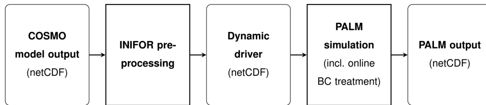
Figure 1. Simulation workflow using PALM’s mesoscale nesting interface.
