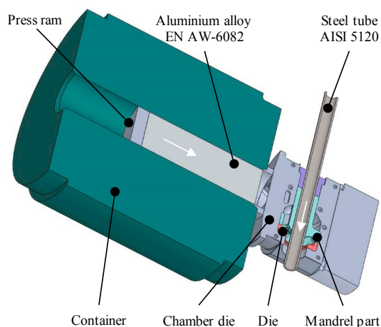
Fig. 1. Cross-section of the 10 MN tool system.
