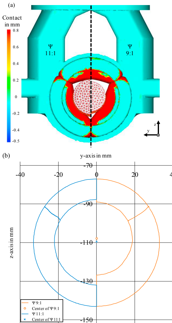
Fig. 6. (a) Stage of contact from the aluminium to the steel rod at a p_i of 89.5 mm left \Psi of 11:1 and right \Psi of 9:1, (b) cross-section of the profile at a p_h of 109.5 mm.
