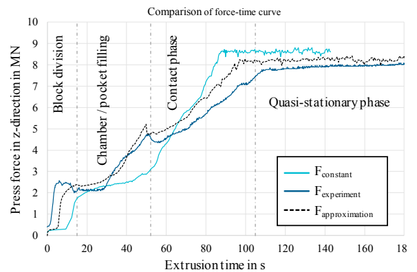
Fig. 11. Comparison of the experimental and numerical force-time curves.
