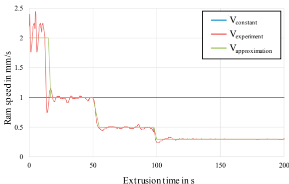
Fig. 10. Experimental and numerical velocity profile.
