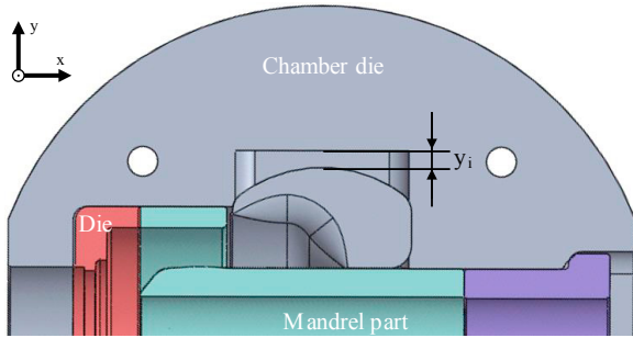
Fig. 2. Cross-section of the chamber die with cavity depth y_i .
