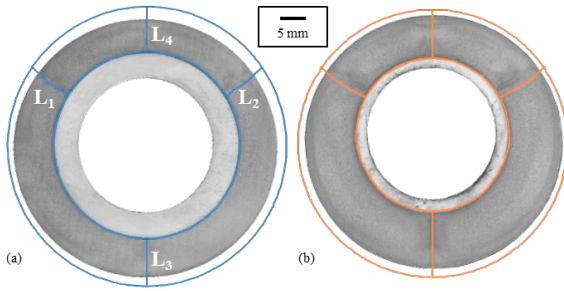
Fig. 9. Comparison of the geometries in the cross-section at a p_h of 109.5 mm (a) \Psi of 11:1 and (b) \Psi of 9:1.
